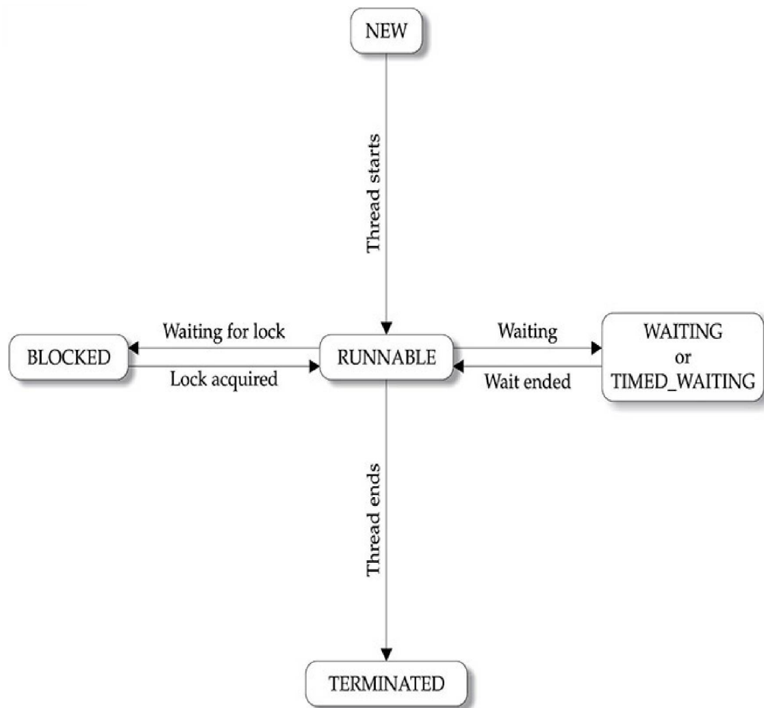
Figure 11-1 diagrams how the various thread states relate.
