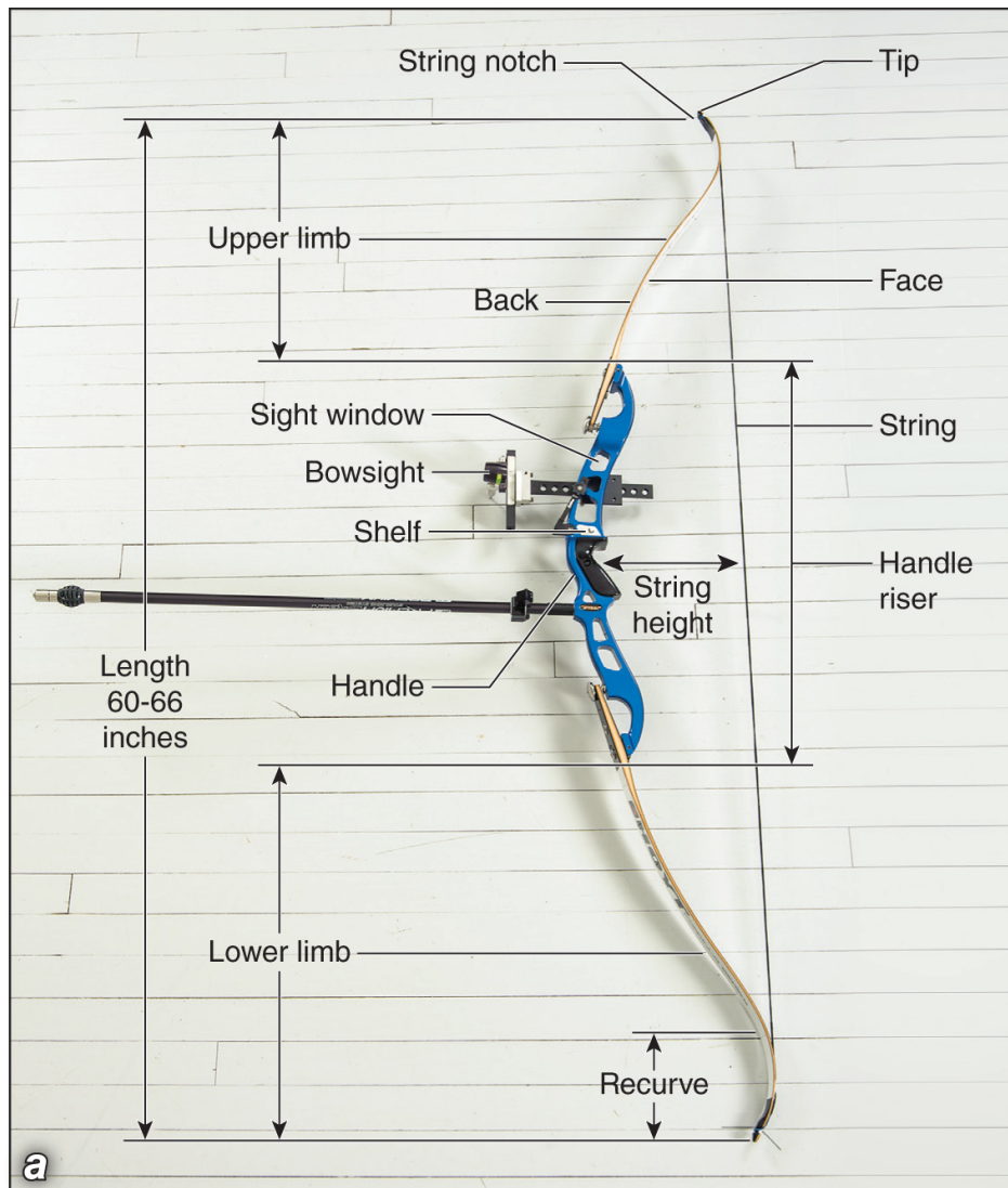
Figure 6 Various views of a recurve bow: (a) bow with major parts labeled.
