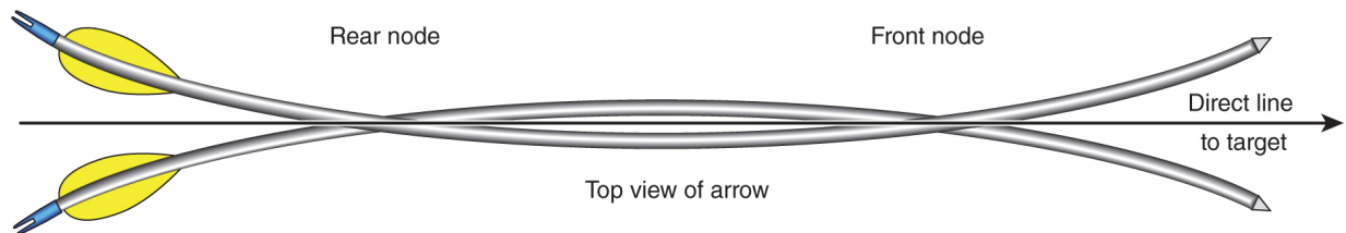
Figure 8.17 On release of the bowstring, the arrow bends, oscillating around two points called nodes.
