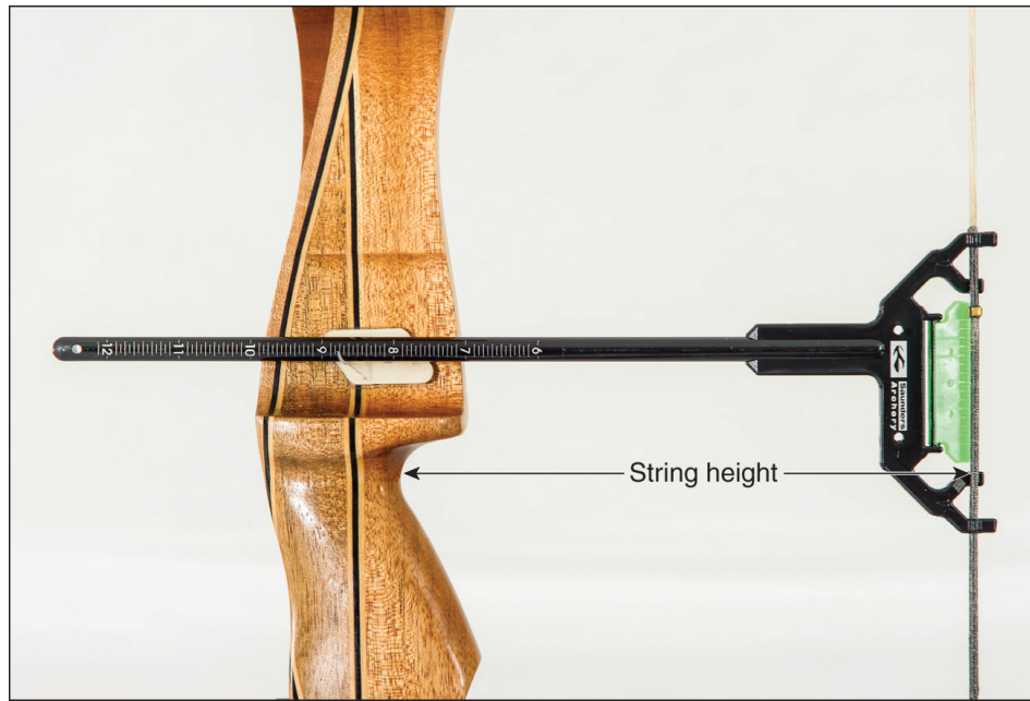
Figure 2.2 A bow square positioned to allow you to check the string, or brace, height.
