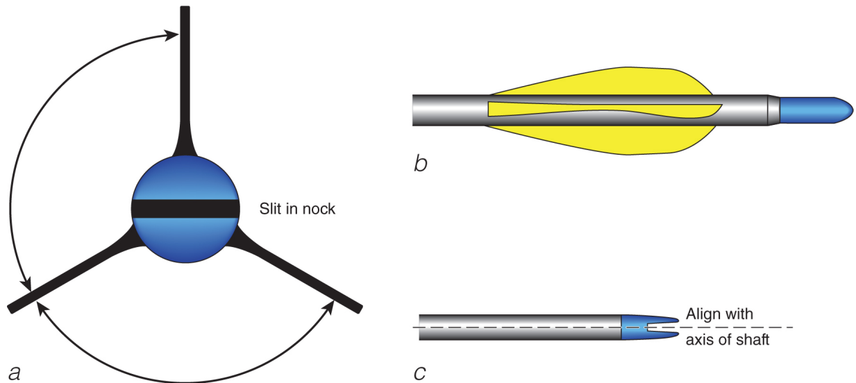
Figure 8.23 Arrow nock: (a) cross-section; (b) mounted on shaft; (c) aligned with axis of shaft.
