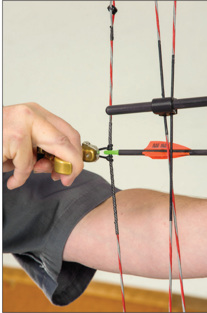
Figure 6.4 Mechanical release looped around the string loop (D loop) rather than around the bowstring.
