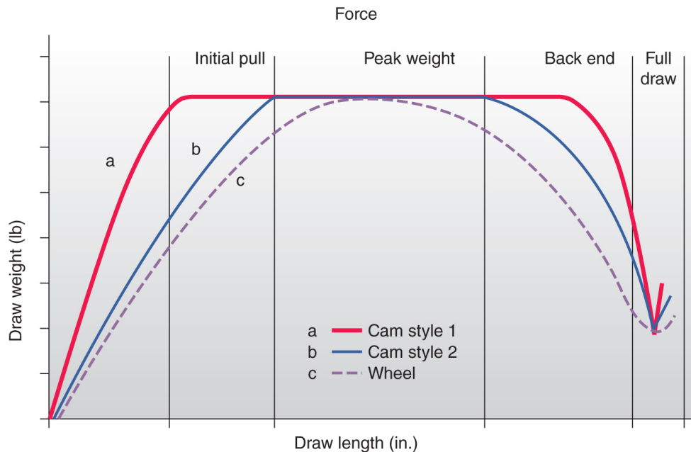
Figure 8.7 A force-draw curve for compound bows. Curves a and b are two styles of cams; the bow is at or near peak weight for a greater portion of the draw and decreases abruptly near full draw. Curve c is a round eccentric (axle off center) wheel; draw weight increases gradually to a peak, decreases gradually, and provides a valley of approximately 1 inch (2.5 cm) or so with minimal holding weight at full draw when matched to an archer's draw length.
