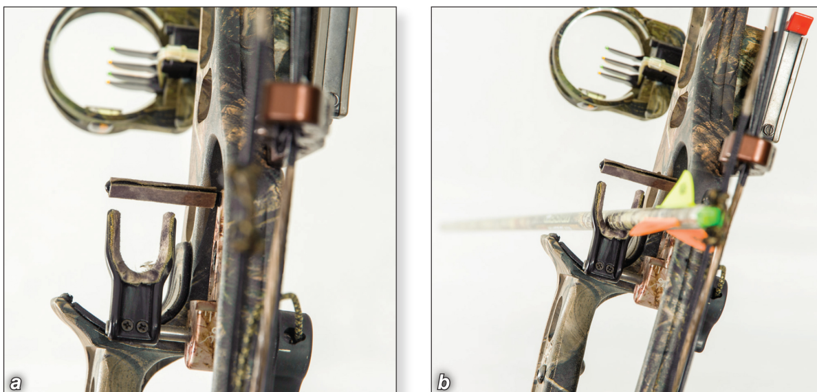
Figure 8.10 A shoot-through rest on a hunting bow. Note that when the arrow is nocked ( b ) the index feather points up.
