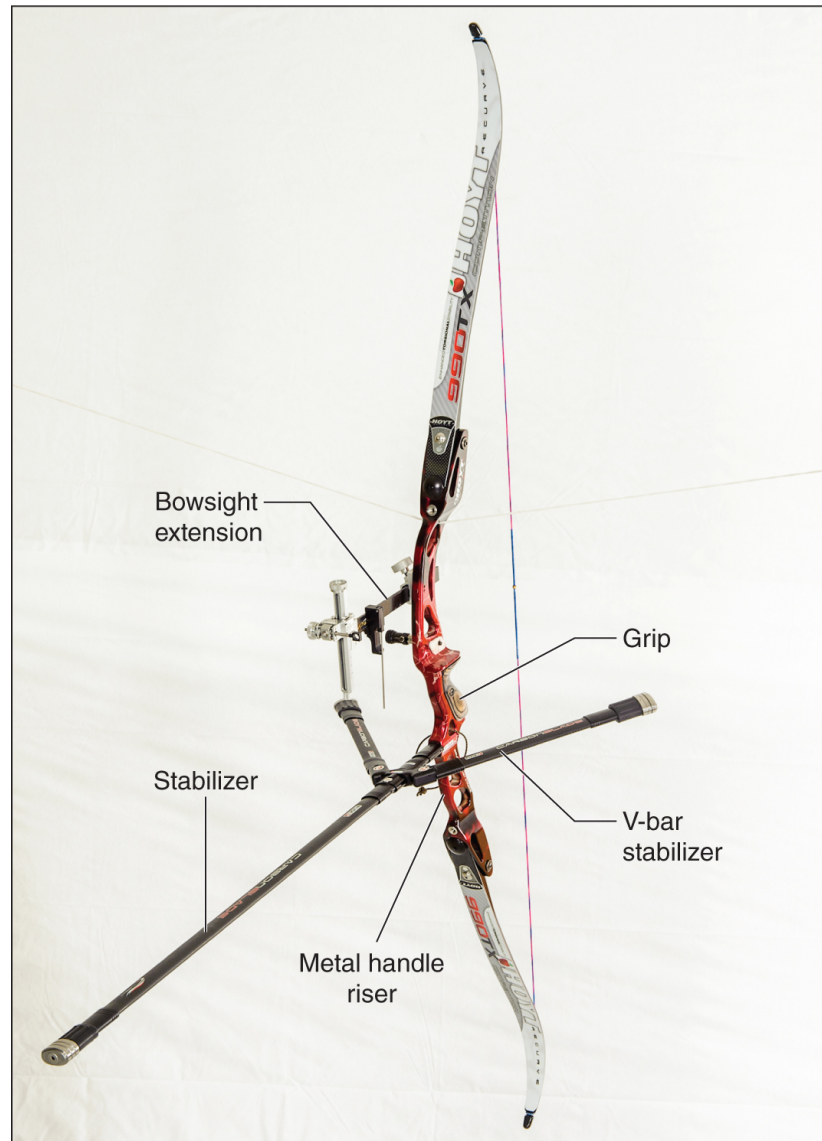
Figure 14 A bow with stabilizer and a bowsight extension attached.
