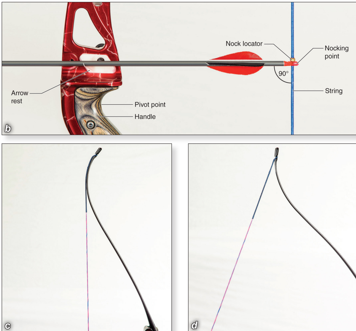
Figure 6 (continued) Various views of a recurve bow: (b) close-up of arrow rest and nocking point area; (c) bow limb in relaxed position; (d) bow limb in drawn position.
