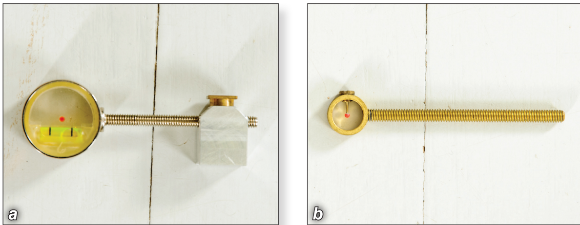
Figure 5.2 Two aiming apertures: (a) aperture with a dot and a level; (b) aperture with a drop-pin.
