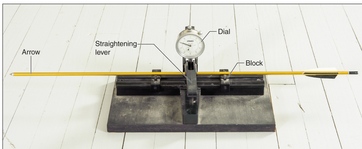
Figure 8.28 An arrow straightener.
