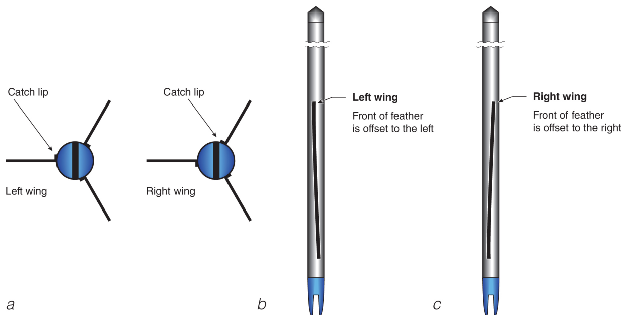
Figure 8.26 (a) Viewing from the nock end, note the location of the catch lip to determine whether your feathers are from a left or right wing. (b) Left-wing feathers are mounted with the front of the feather to the left; (c) right-wing feathers are mounted with the front of the feather to the right.
