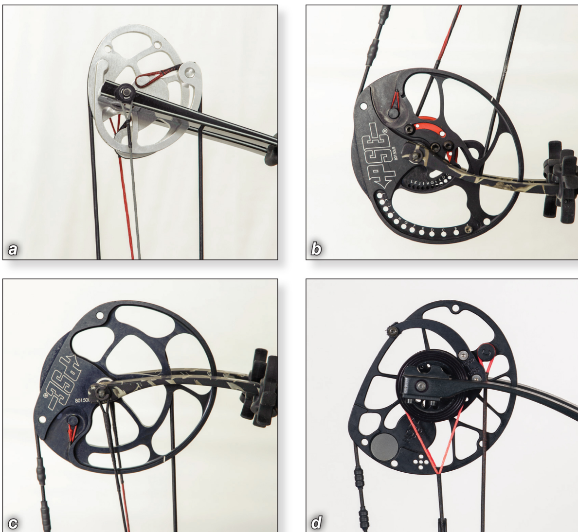
Figure 8.8 Various cam styles.
