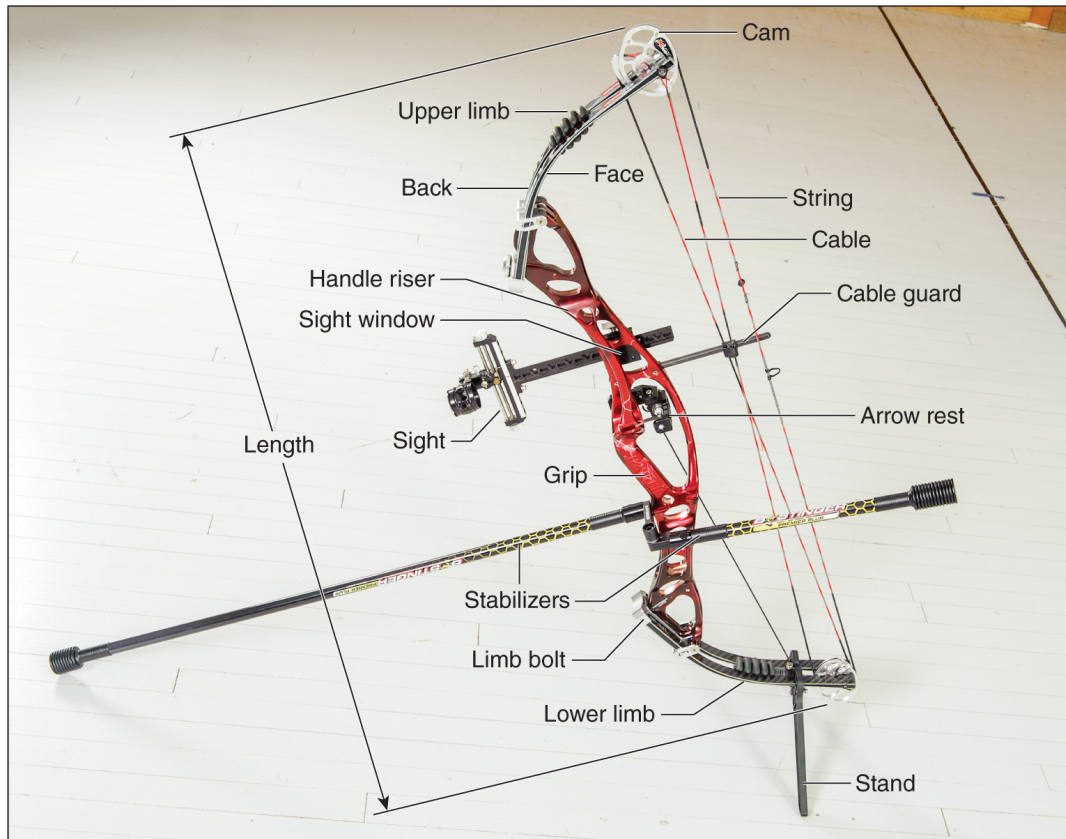
Figure 7 A compound bow. The wheels can be round, eccentric pulleys, or cams.
