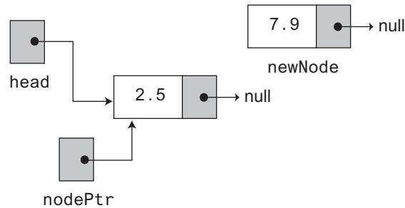
Figure 18-6 nodePtr points to the first node
