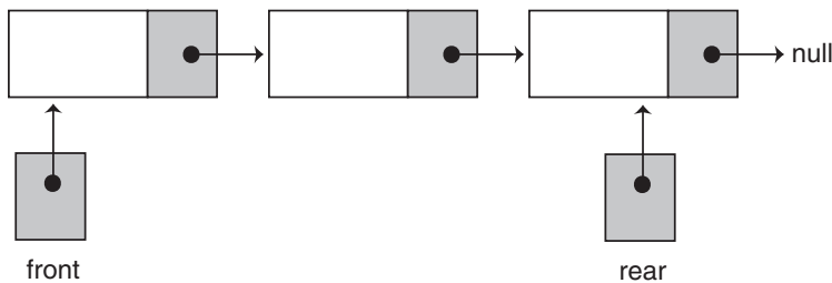
Figure 19-14 A dynamic queue
