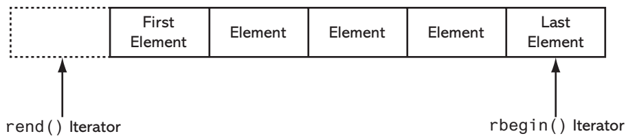
Figure 17-2 Iterators returned by the rbegin() and rend() member functions
