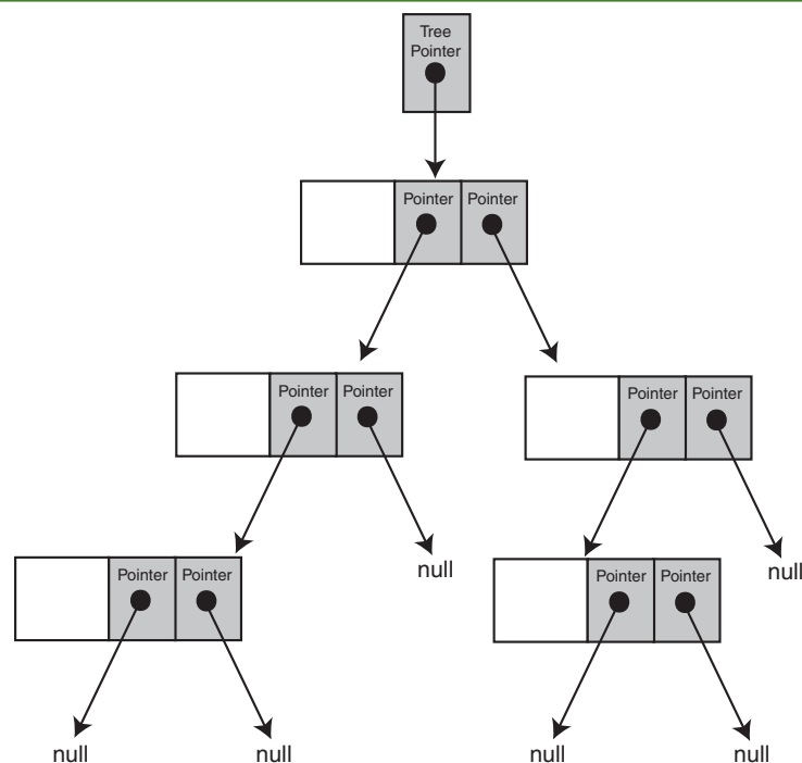
Figure 21-1 A binary tree
