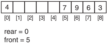
Figure 19-13 The rear of the queue wraps around to the beginning
