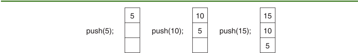
Figure 19-2 State of the stack
