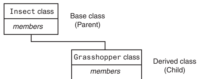
Figure 15-2 Base class and derived class
