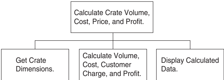
Figure 3-7 Hierarchy chart for the program
