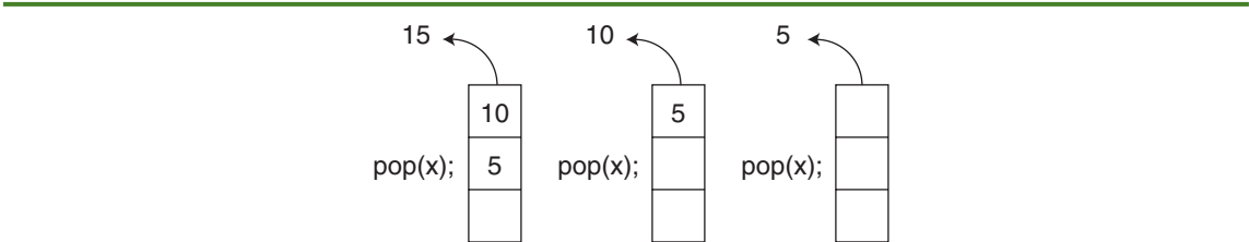
Figure 19-3 State of the stack
