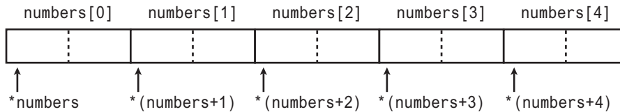
Figure 9-6 Subscript notation and pointer notation
