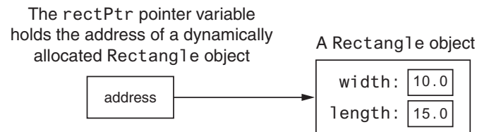
Figure 13-12 rectPtr points to a dynamically allocated Rectangle object
