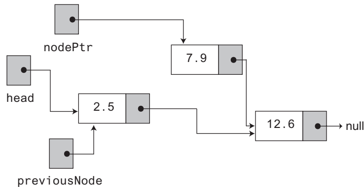
Figure 18-18 Node removed from the list
