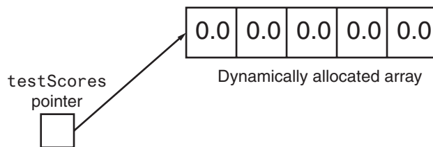
Figure 14-3 The testScores member referencing a dynamically allocated array
