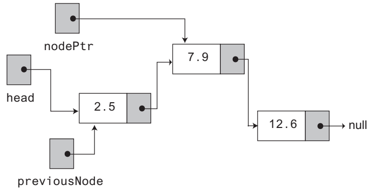
Figure 18-17 previousNode points to the first node and nodePtr points to the second node
