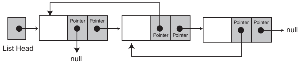
Figure 18-19 A doubly linked list
