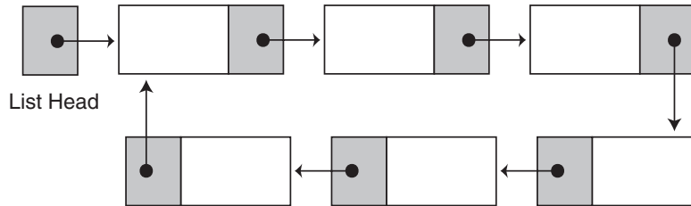
Figure 18-20 A circularly linked list
