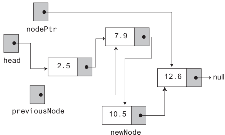
Figure 18-15 The new node inserted
