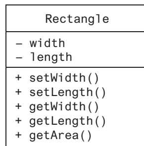
Figure 13-20 Rectangle class with access specification
