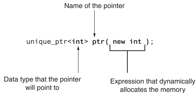
Figure 9-12 Definition of a unique_ptr
