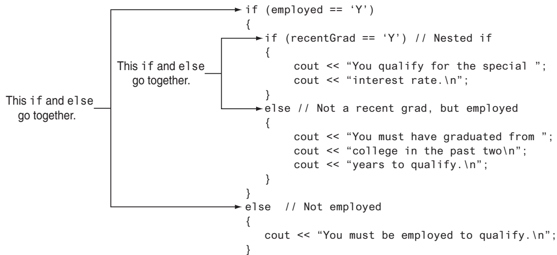
Figure 4-8 Proper indentation and alignment
