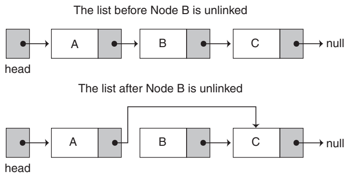
Figure 18-16 Unlinking a node
