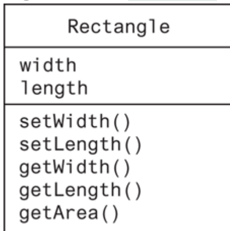
Figure 13-19 Rectangle class
