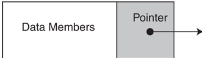
Figure 18-1 A node
