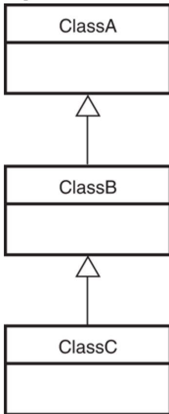
Figure 15-4 Class hierarchy
