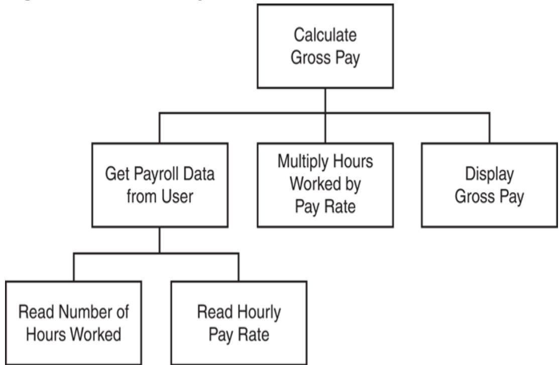
Figure 1-12 Hierarchy chart
