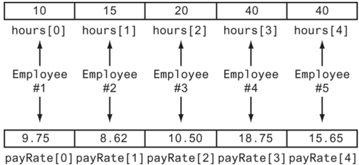
Figure 7-13 Parallel arrays
