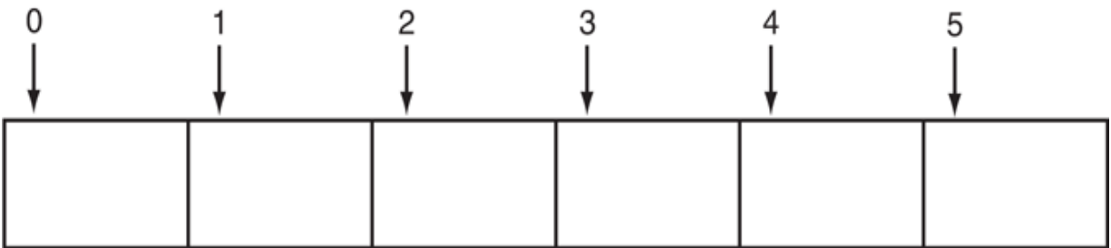
Figure 7-4 Subscripts Subscripts
