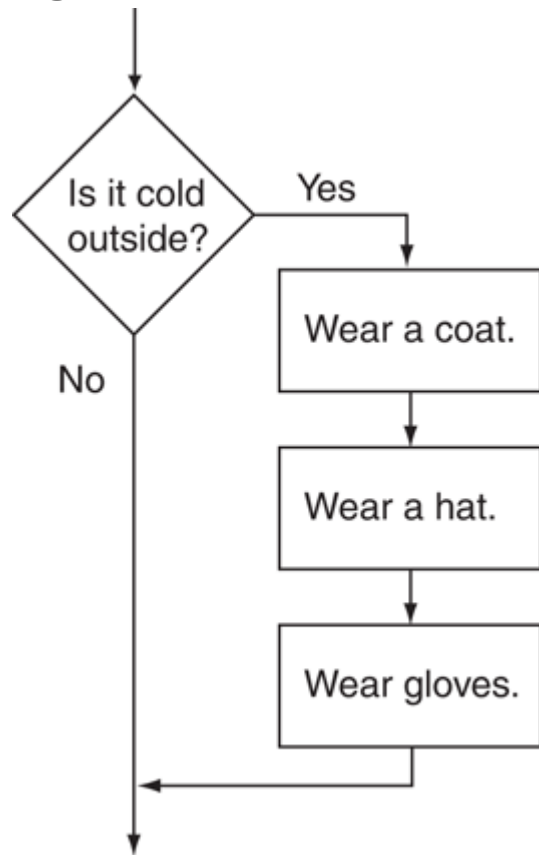
Figure 4-3 Decision structure
