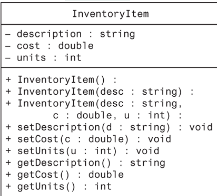
Figure 13-22 InventoryItem class
