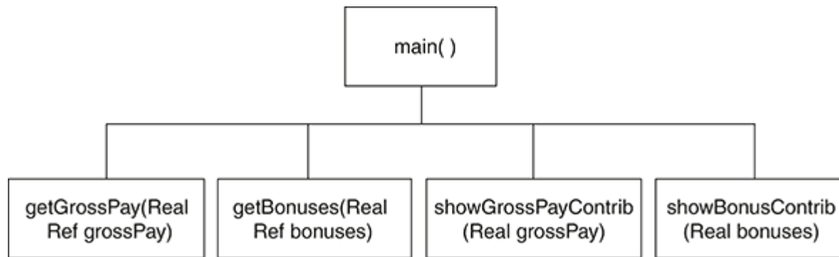
Figure 3-20 Hierarchy chart
