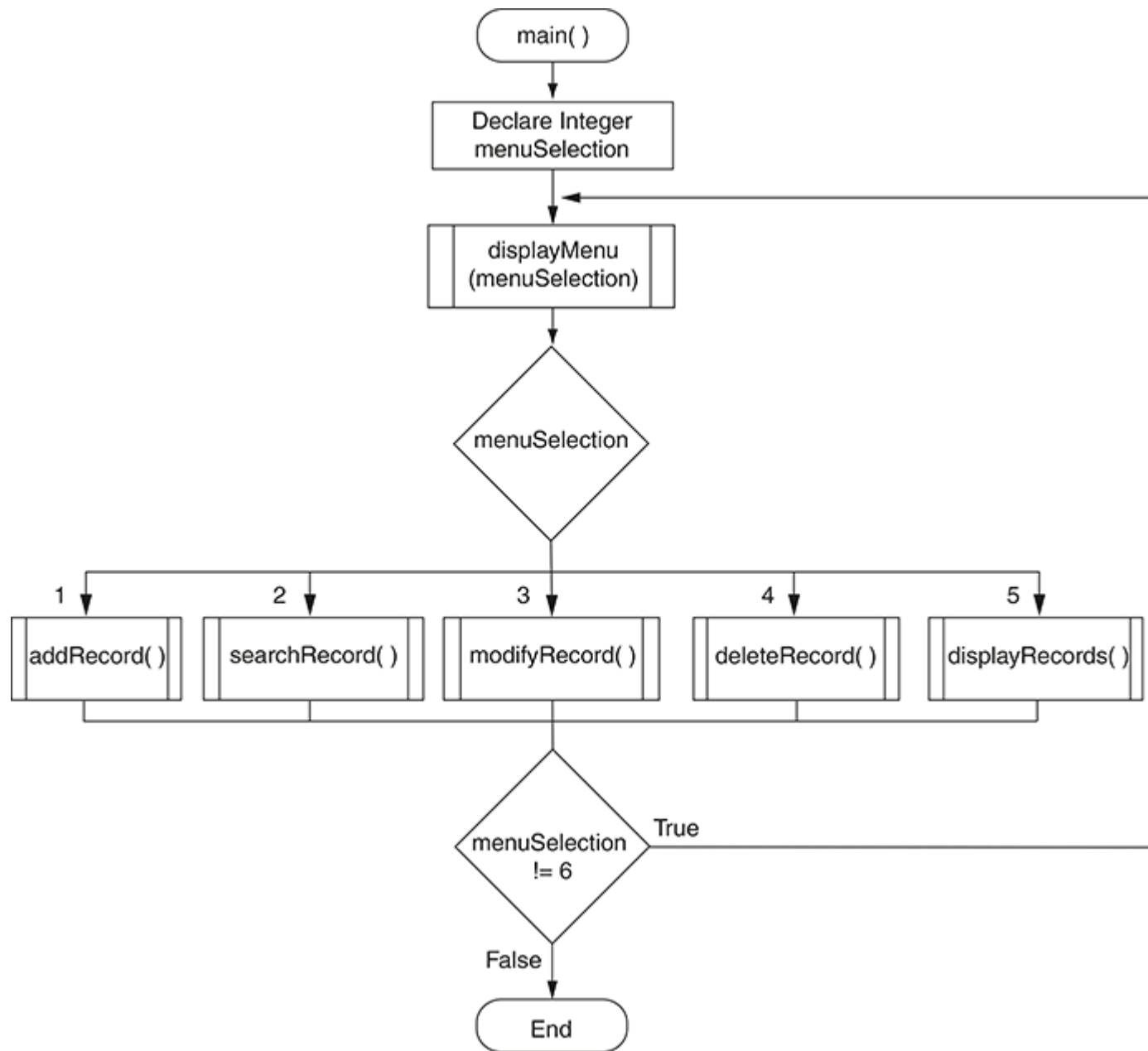
Figure 11-8 Flowchart for the main module in Program 11-6
