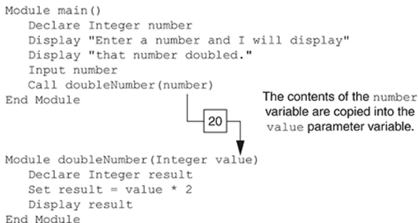
Figure 3-13 The contents of the number variable passed as an argument
