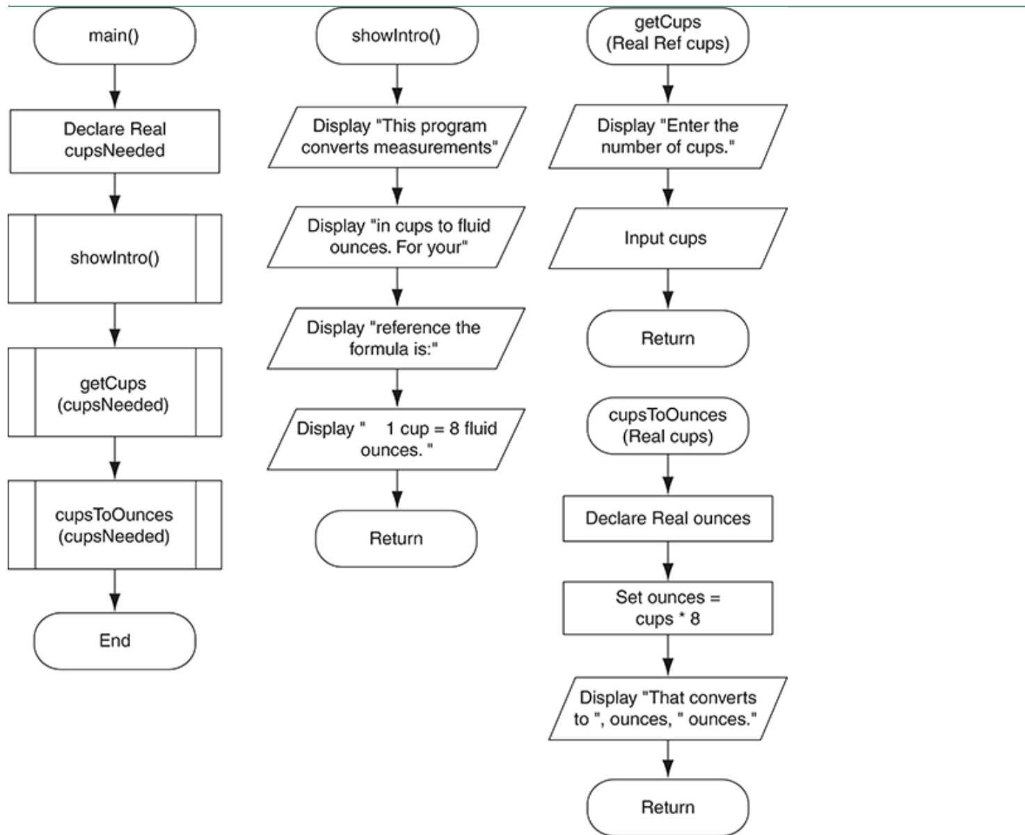
Figure 3-19 Flowchart for Program 3-11
