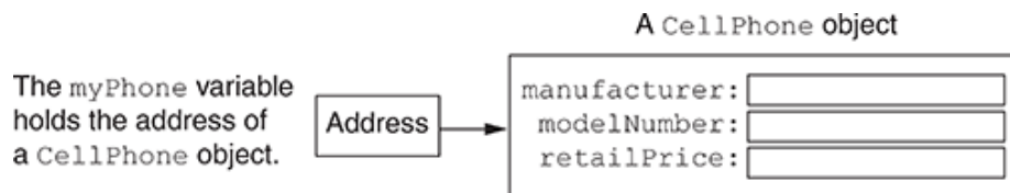
Figure 14-8 The myPhone variable references a CellPhone object
