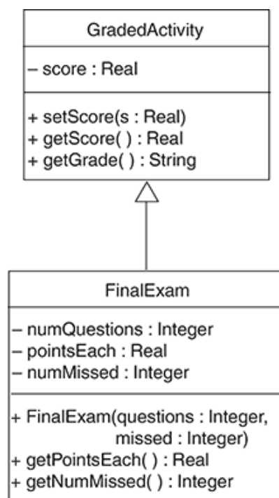
Figure 14-20 UML diagram showing inheritance
