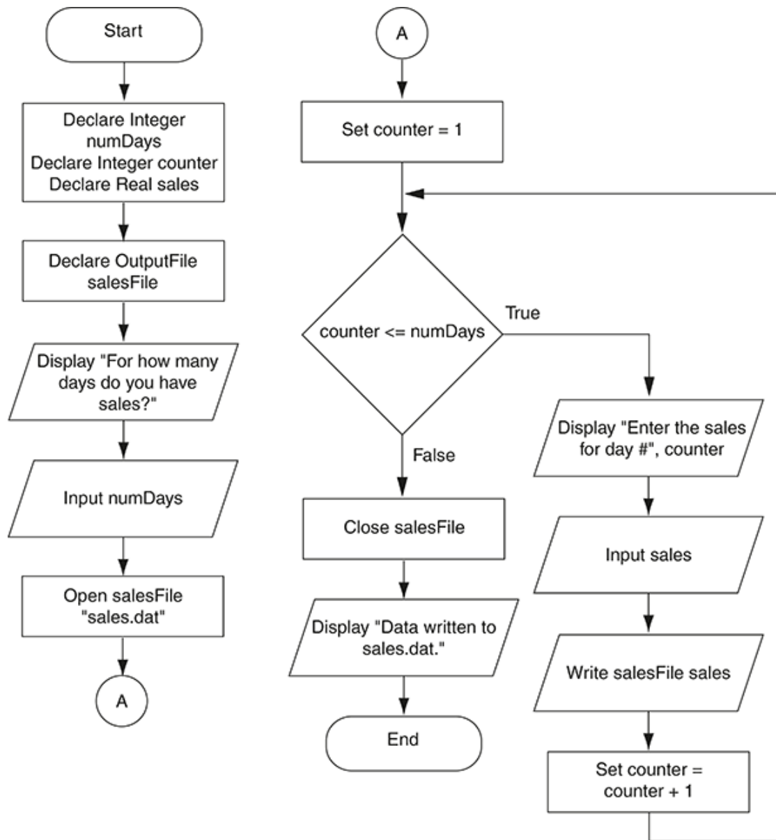
Figure 10-13 Flowchart for Program 10-3
