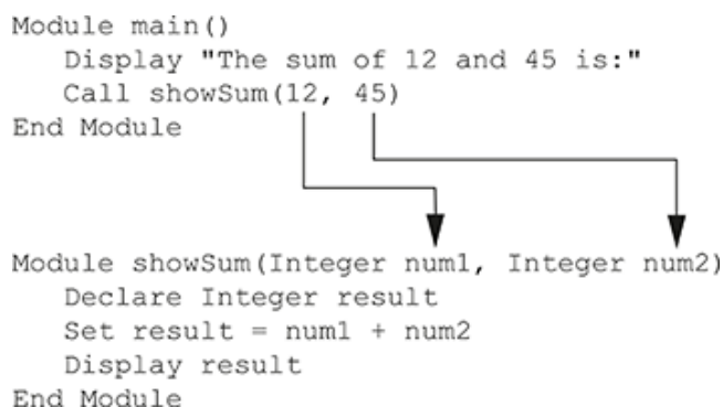
Figure 3-15 Two arguments passed into two parameters
