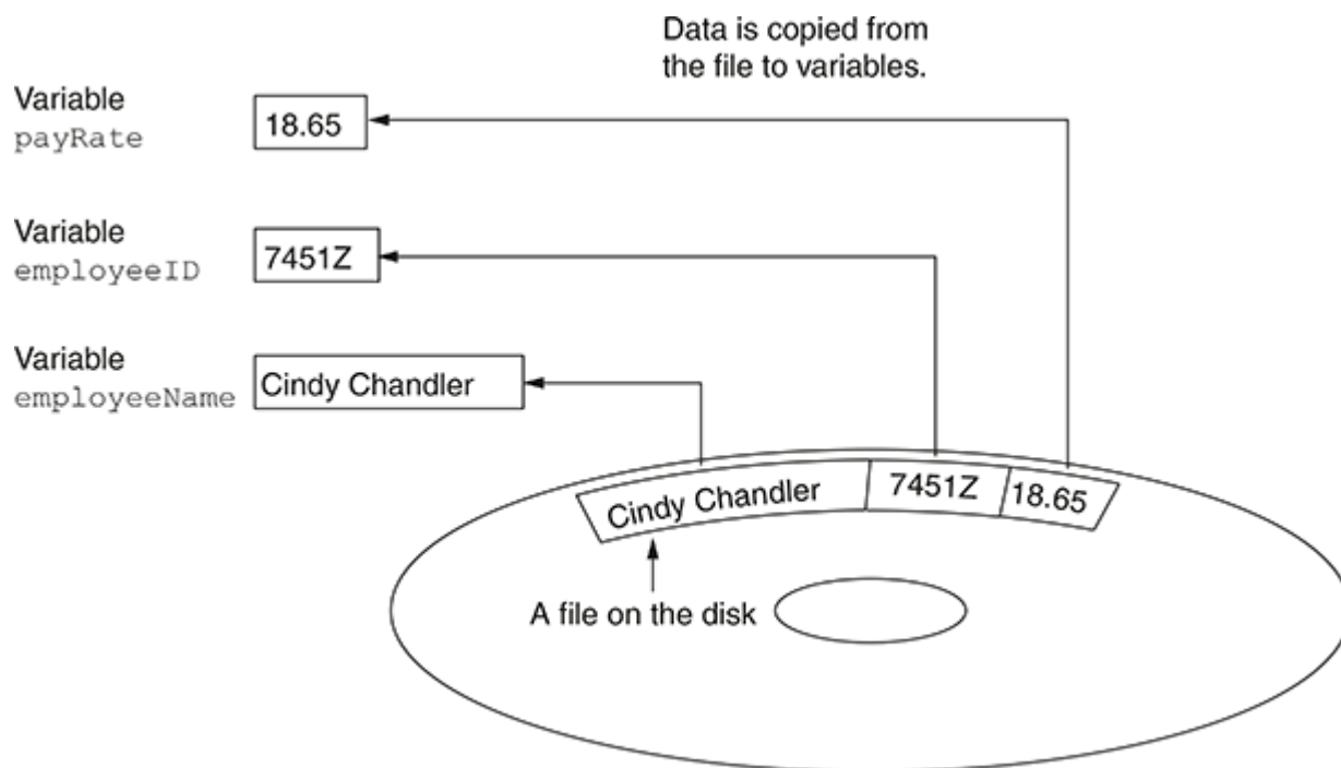
Figure 10-2 Reading data from a file
