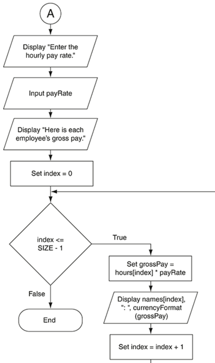
Figure 8-15
