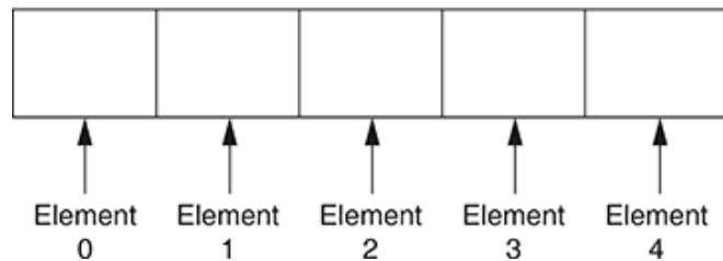
Figure 8-1 Array subscripts
