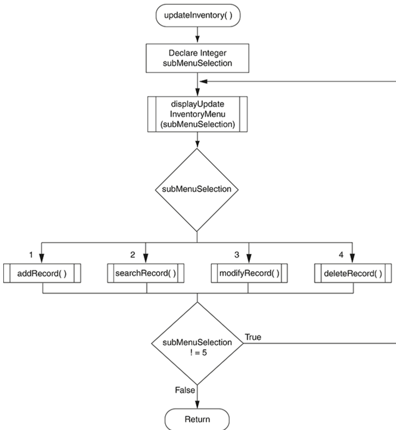
Figure 11-18 Logic for the updateInventory module
