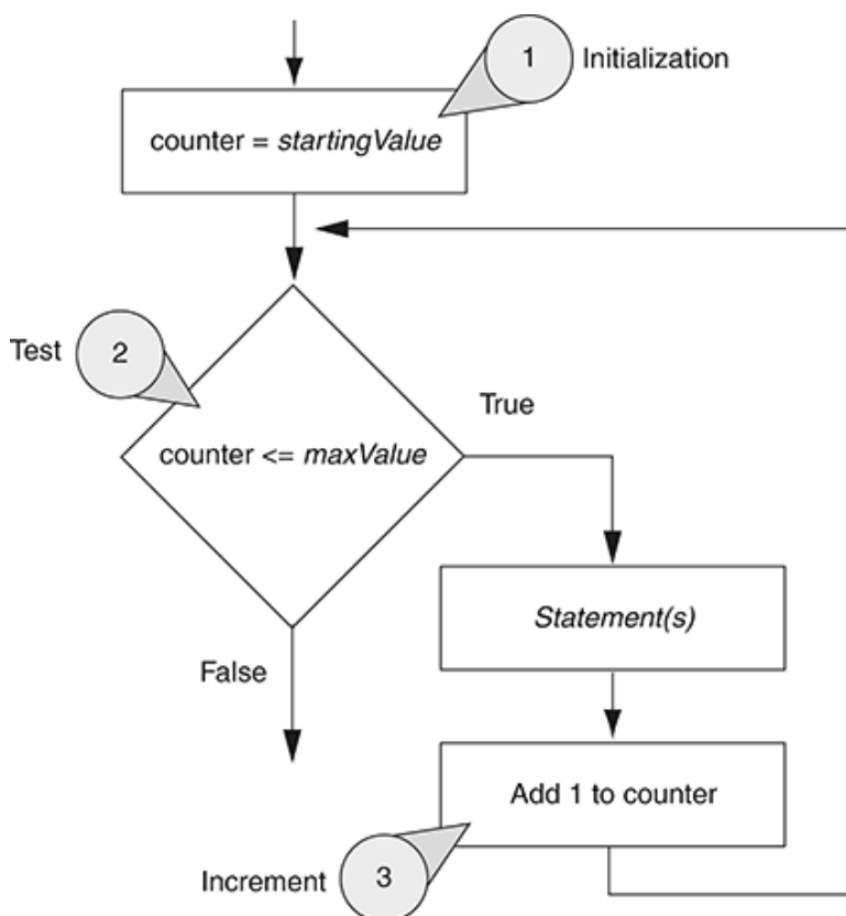
Figure 5-12 Logic of a count-controlled loop
