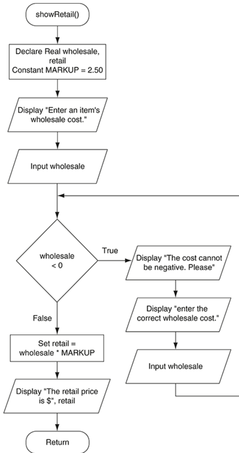
Figure 7-2 Flowchart for the showRetail module
