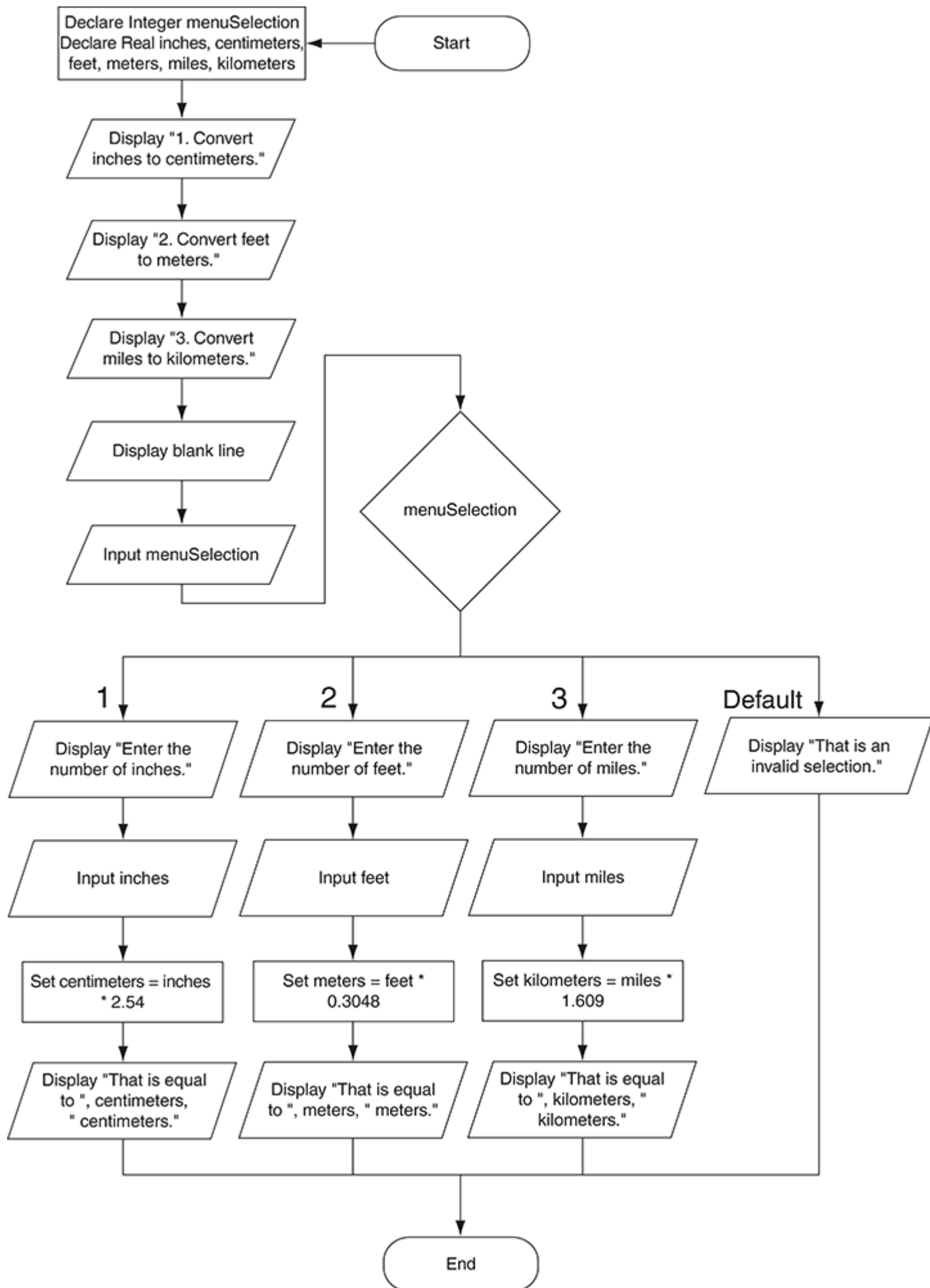
Figure 11-2 Flowchart for Program 11-1
