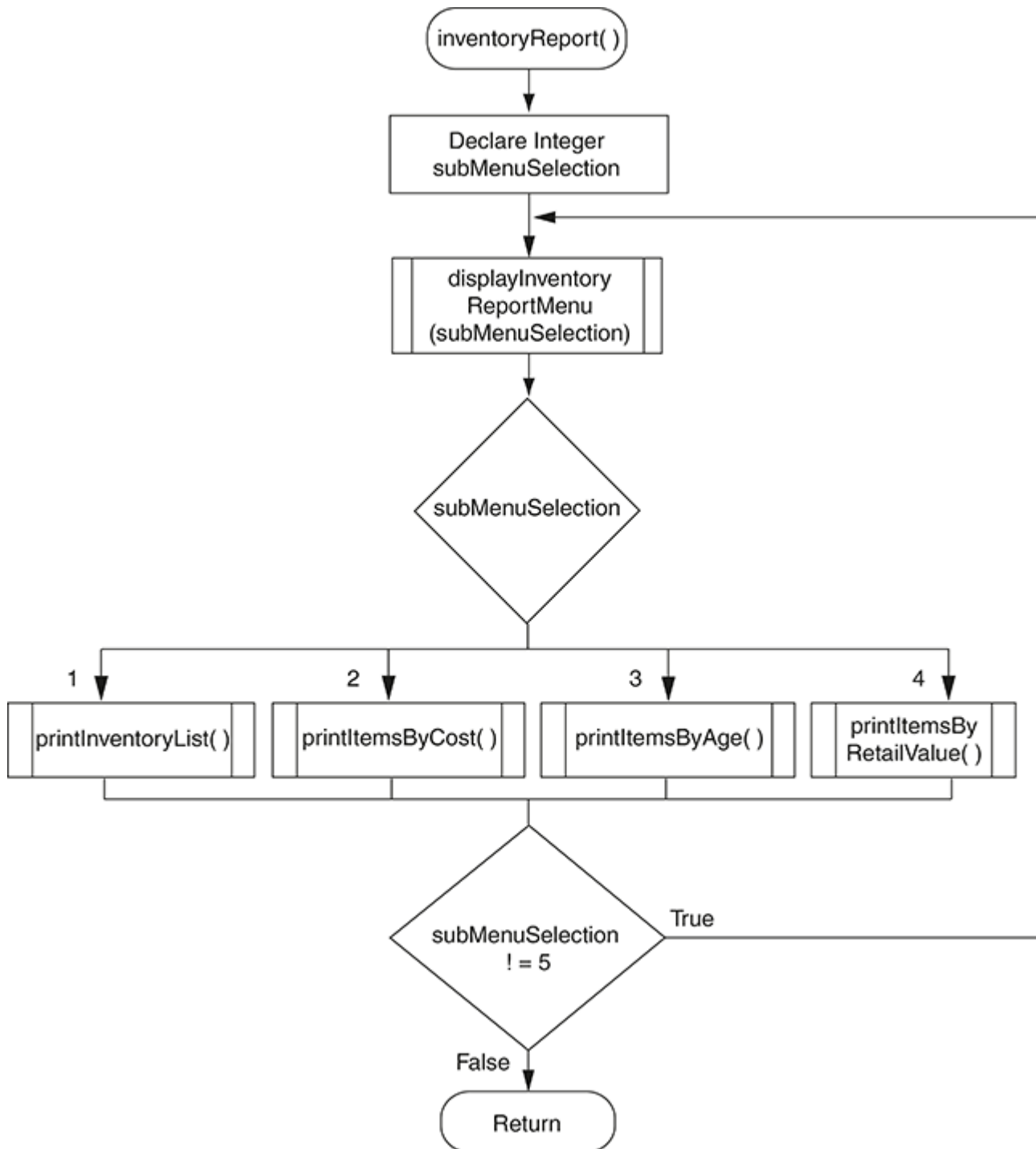
Figure 11-19 Logic for the inventoryReport module
