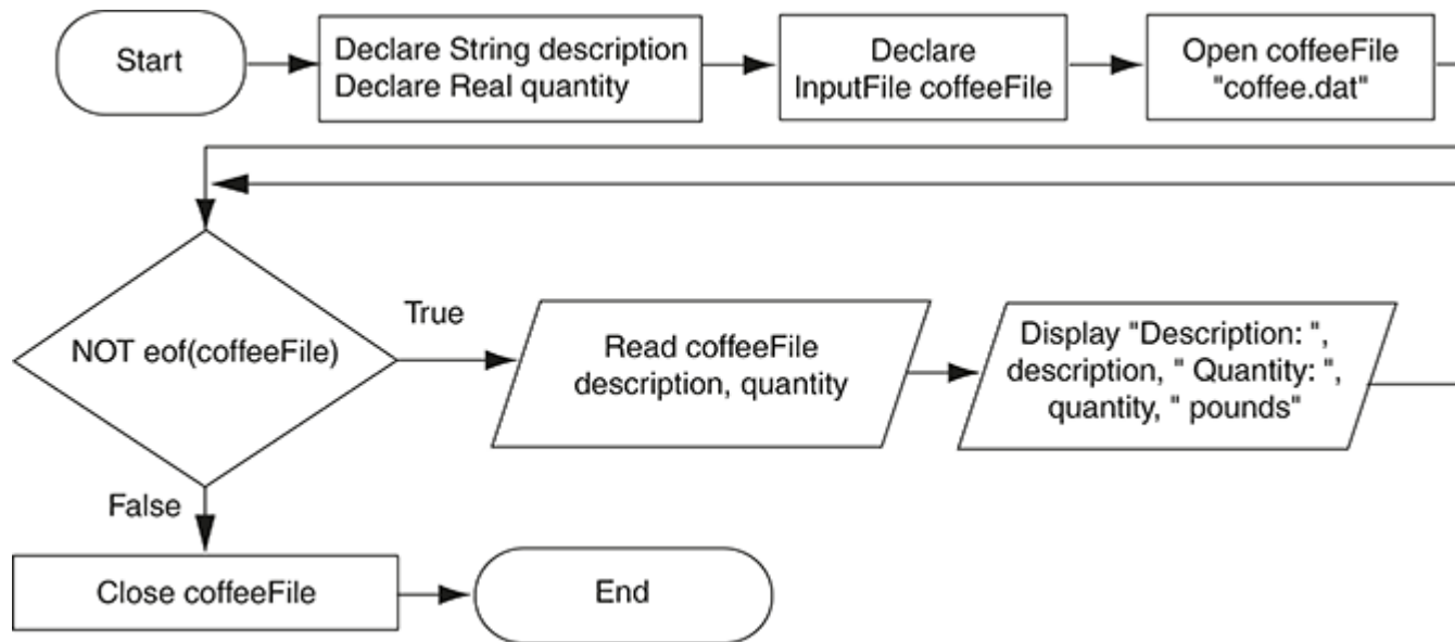
Figure 10-22 Flowchart for Program 10-10
