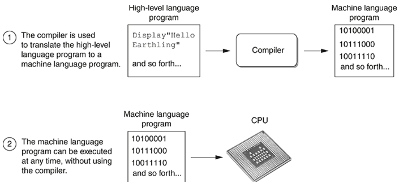
Figure 1-18 Compiling a high-level program and executing it
