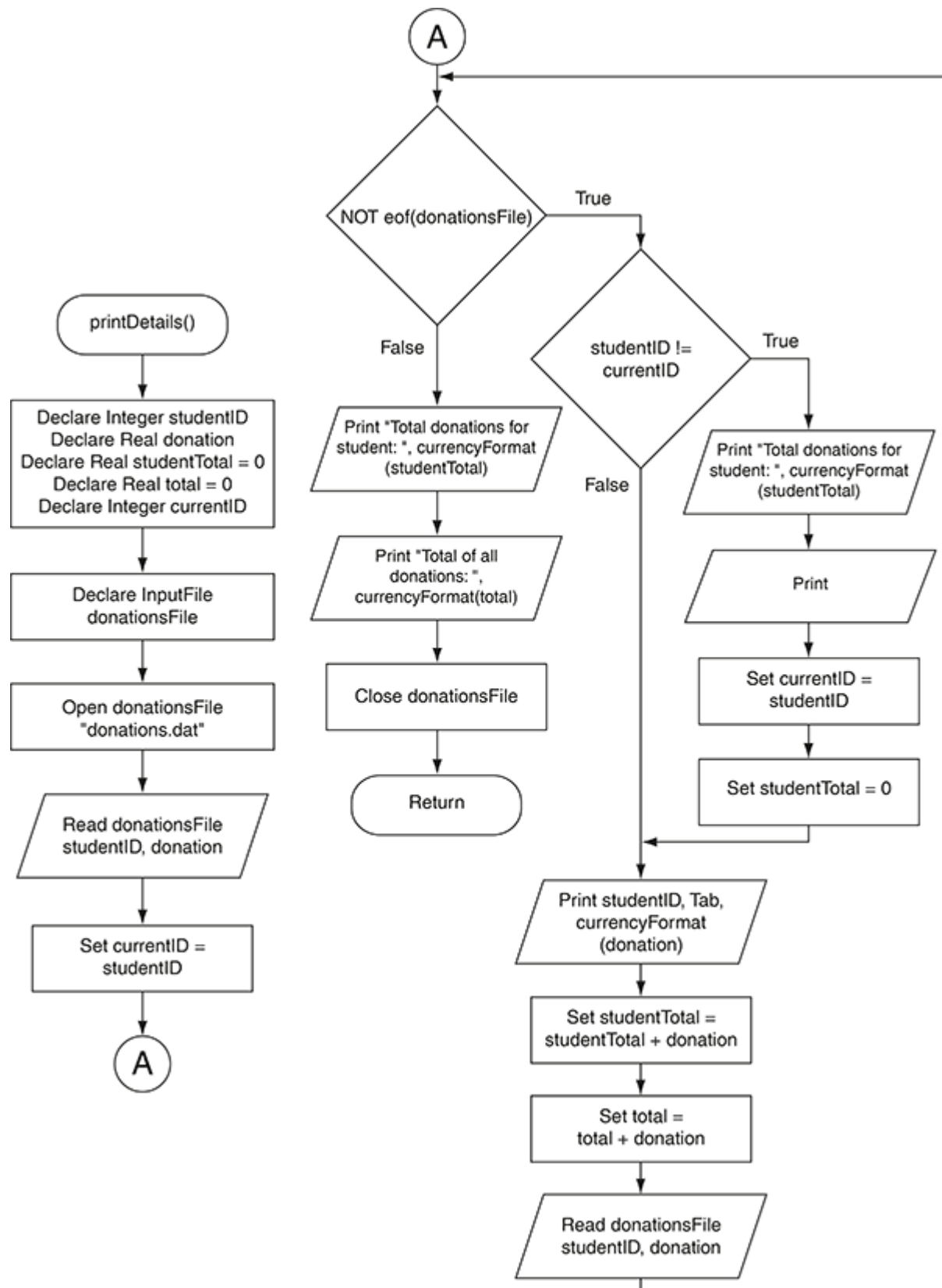
Figure 10-28 Flowchart for the printDetails module
