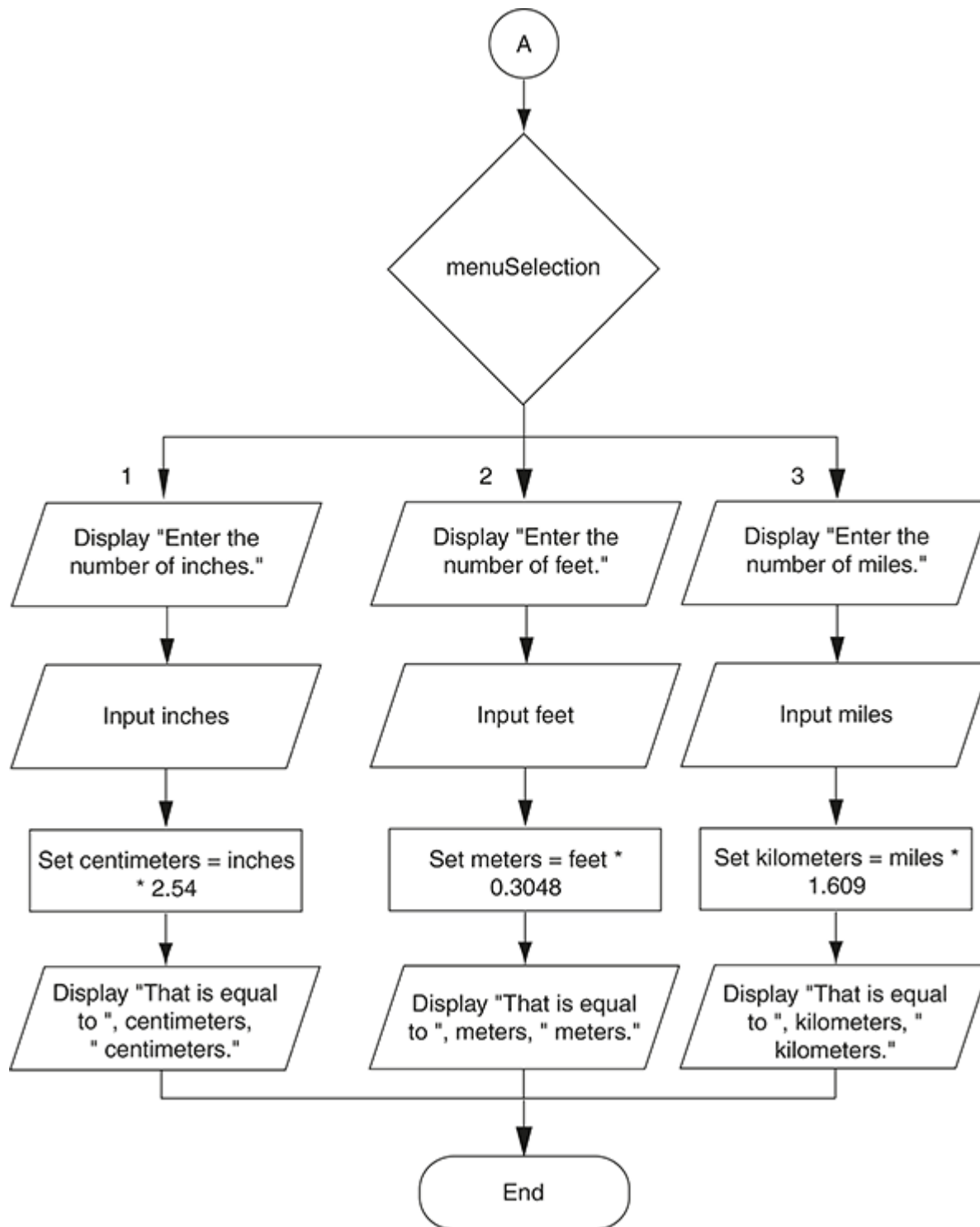
Figure 11-4 Flowchart for Program 11-3
