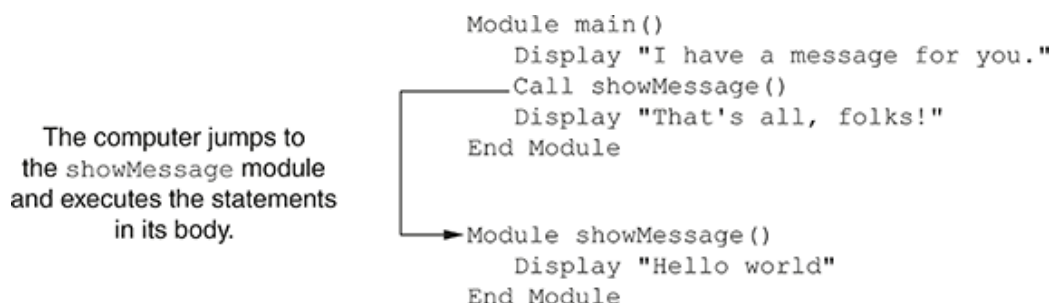
Figure 3-3 Calling the showMessage module
