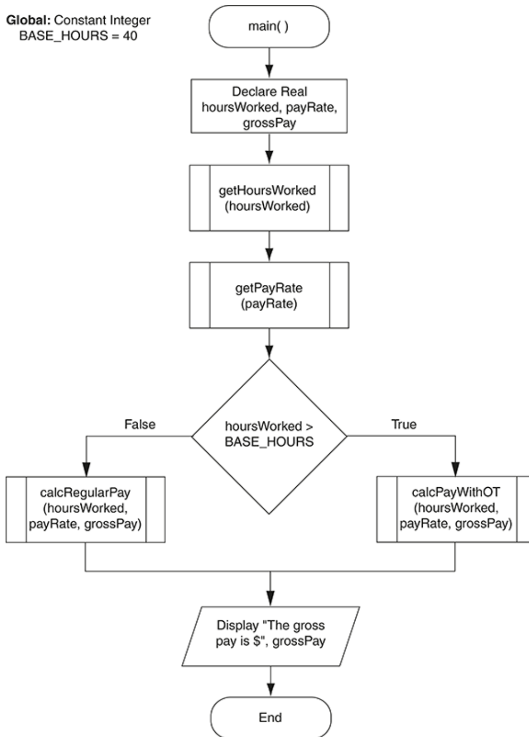
Figure 4-11 Flowchart for the main module
