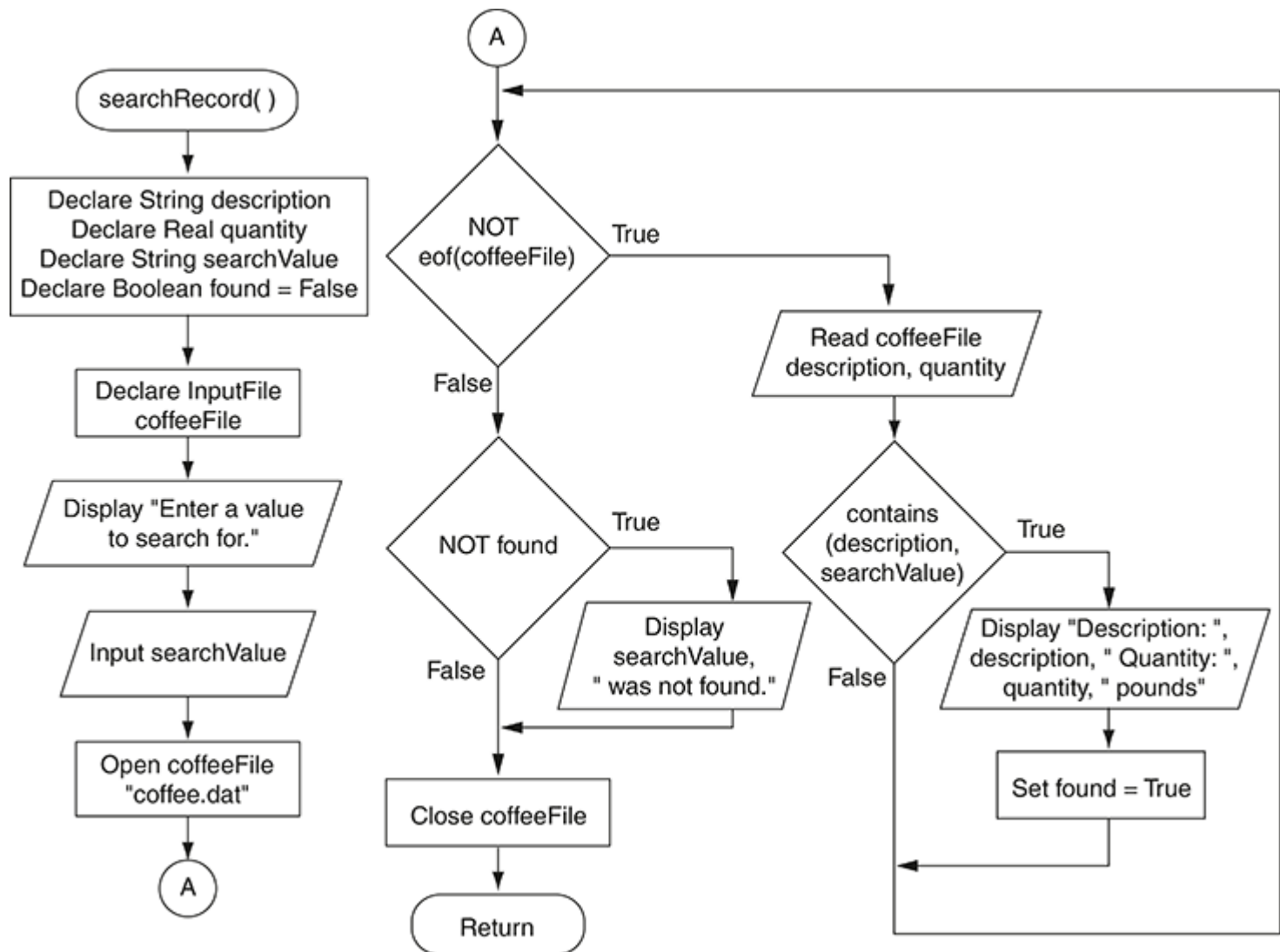
Figure 11-11 Flowchart for the searchRecord module in Program 11-6
