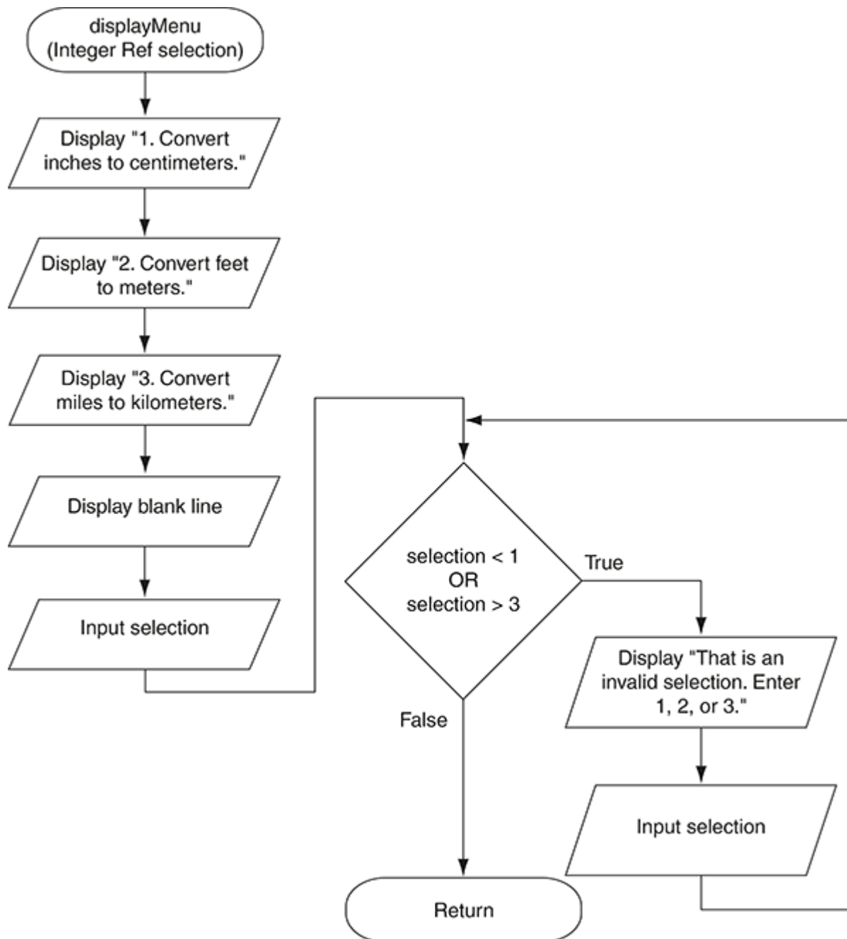
Figure 11-6 Flowcharts for the other modules in Program 11-4
