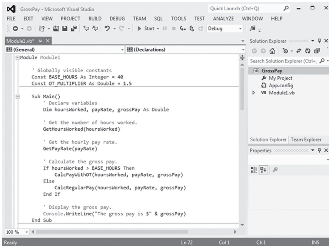
Figure 1-20 An integrated development environment
