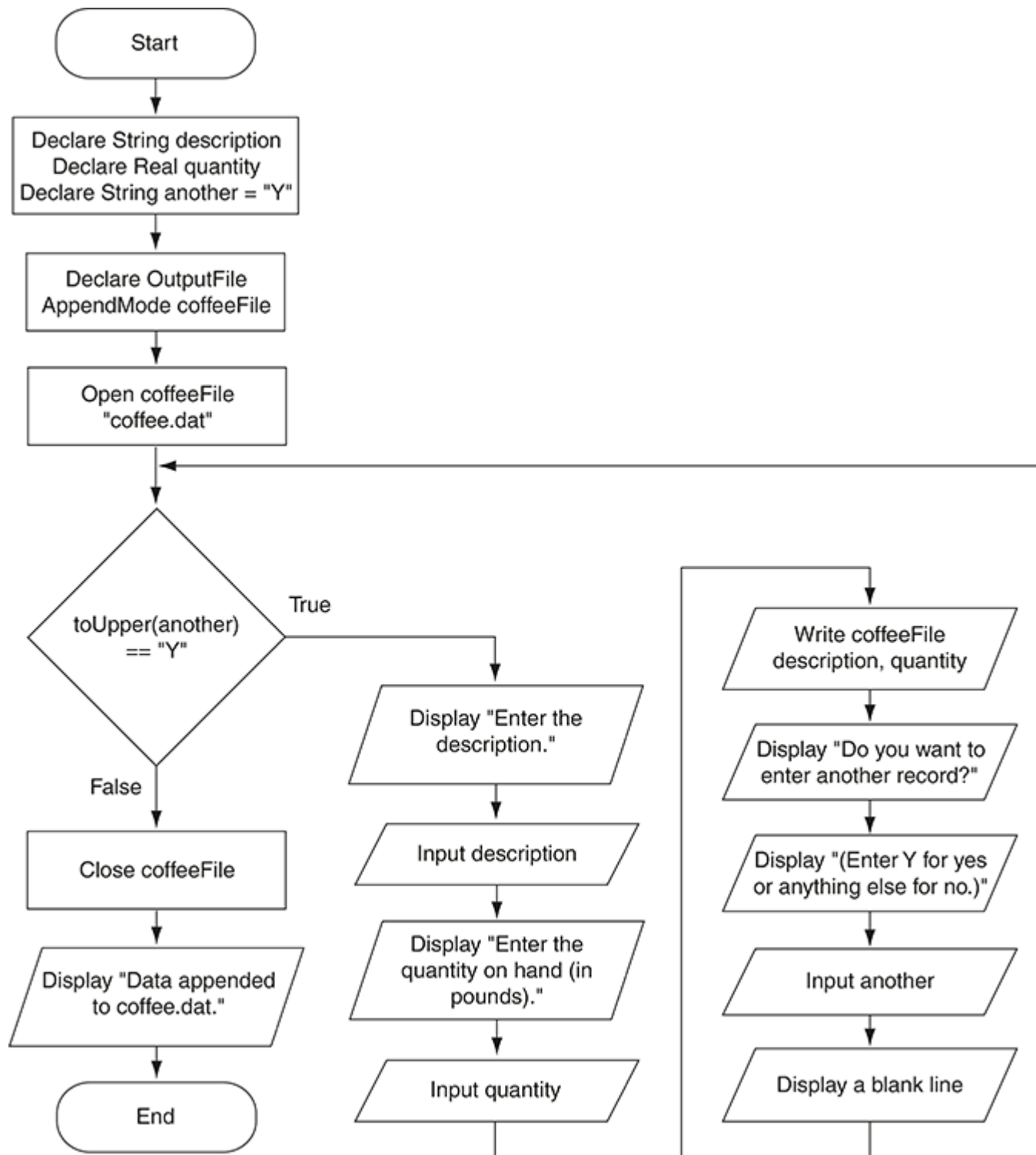
Figure 10-21 Flowchart for Program 10-9
