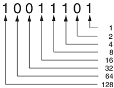
Figure 1-9 The values of binary digits
