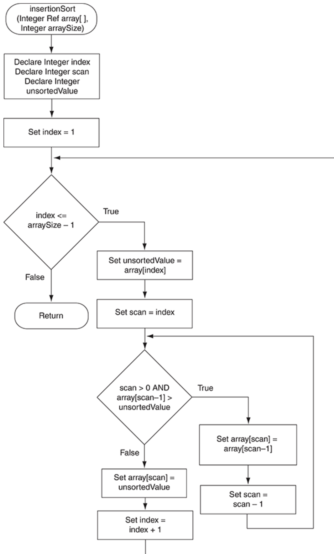
Figure 9-24 Flowchart for the insertionSort module
