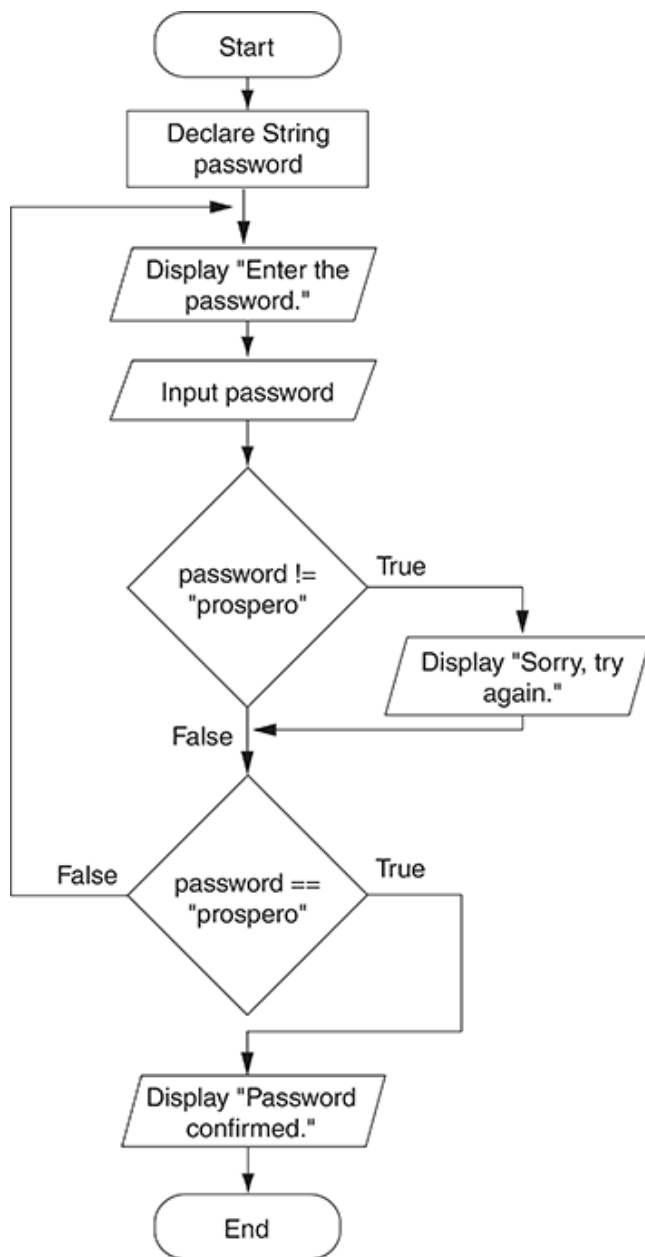
Figure 5-11 Flowchart for Program 5-7
