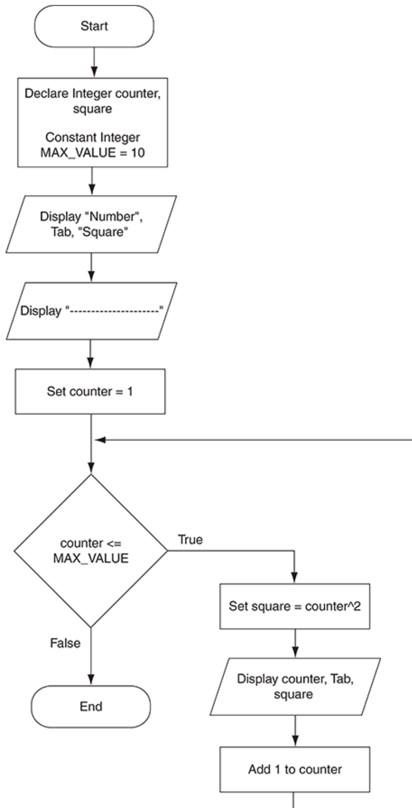
Figure 5-15 Displaying the numbers 1 through 10 and their squares
