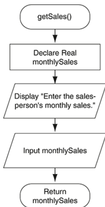
Figure 6-12 Flowchart for the getSales function
