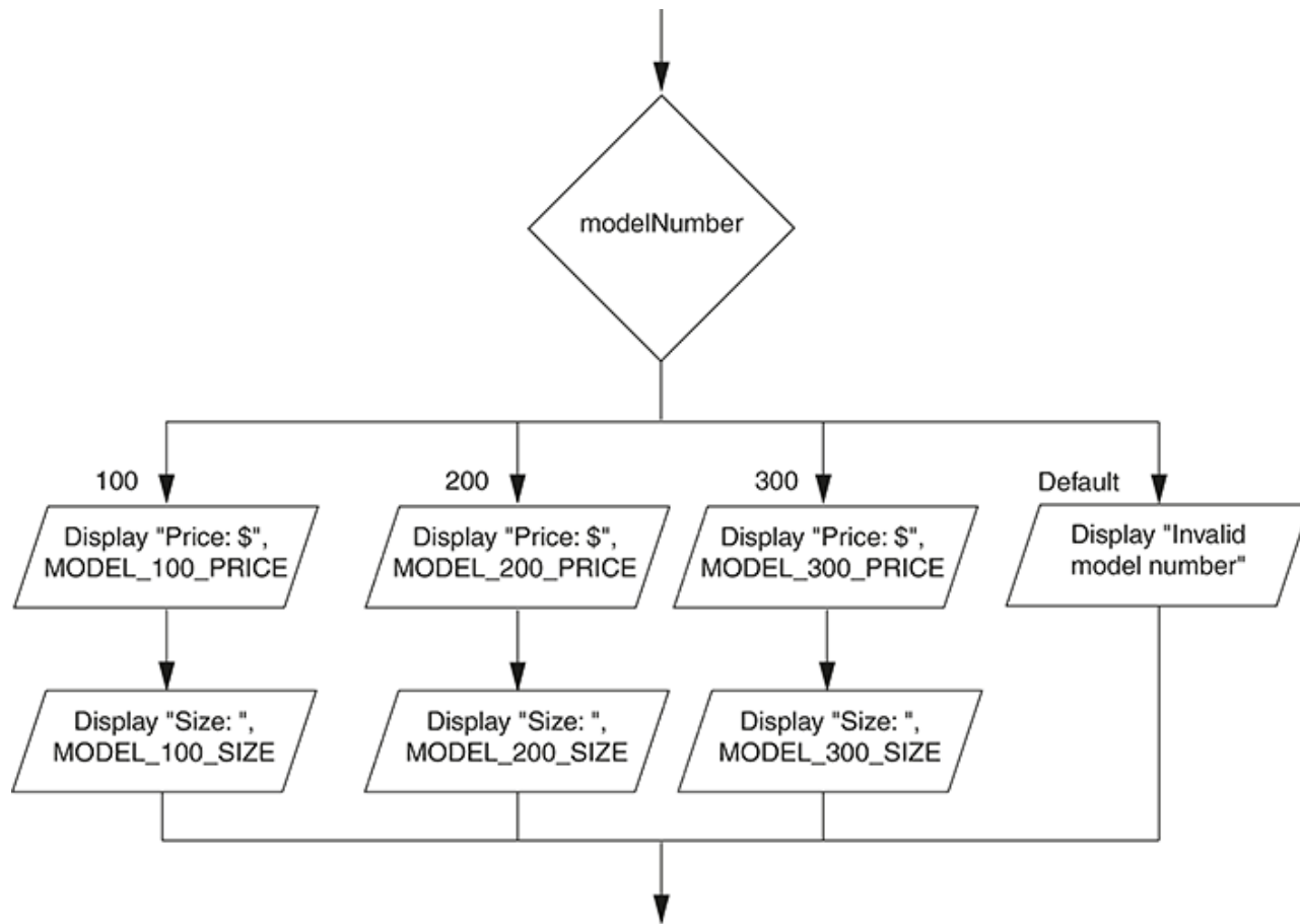
Figure 4-20 Flowchart for the case structure
