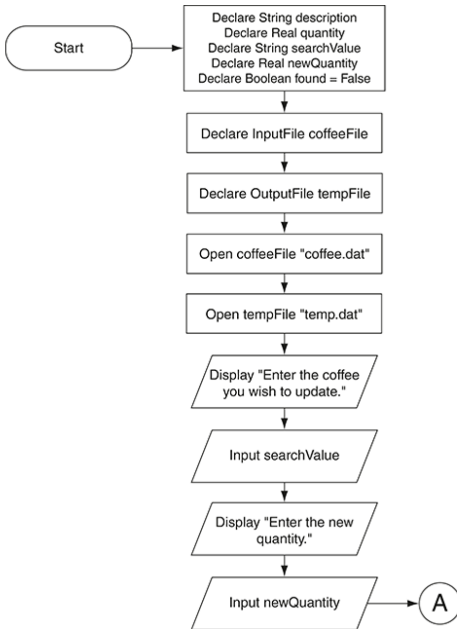
Figure 10-24 Flowchart for Program 10-12, part 1
