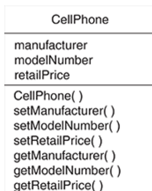
Figure 14-11 Simplified UML diagram for the CellPhone class
