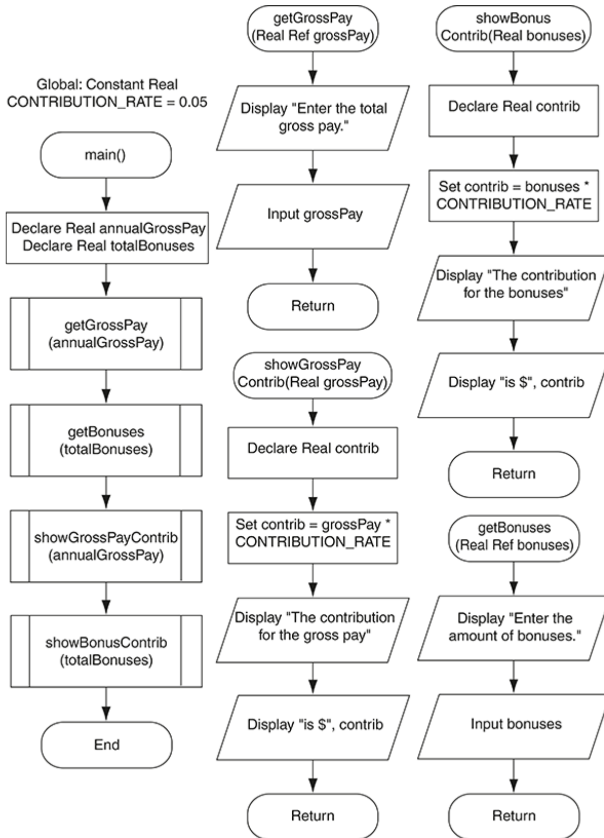
Figure 3-21 Flowchart for Program 3-13
