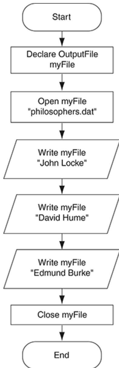
Figure 10-4 Flowchart for Program 10-1
