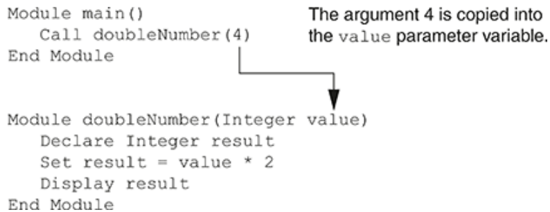
Figure 3-12 The argument 4 is copied into the value parameter variable
