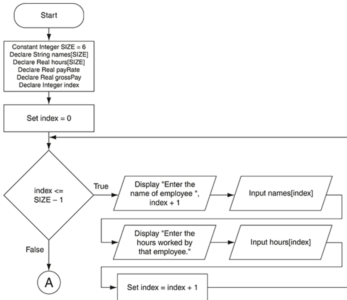
Figure 8-15 Flowchart for Program 8-15
