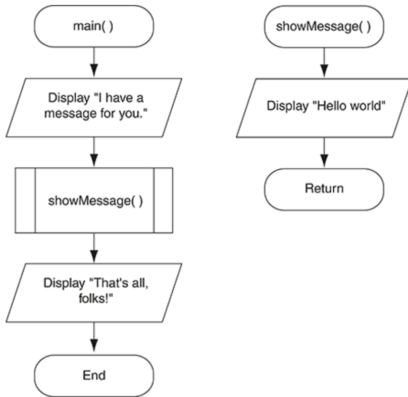
Figure 3-6 Flowchart for Program 3-1
