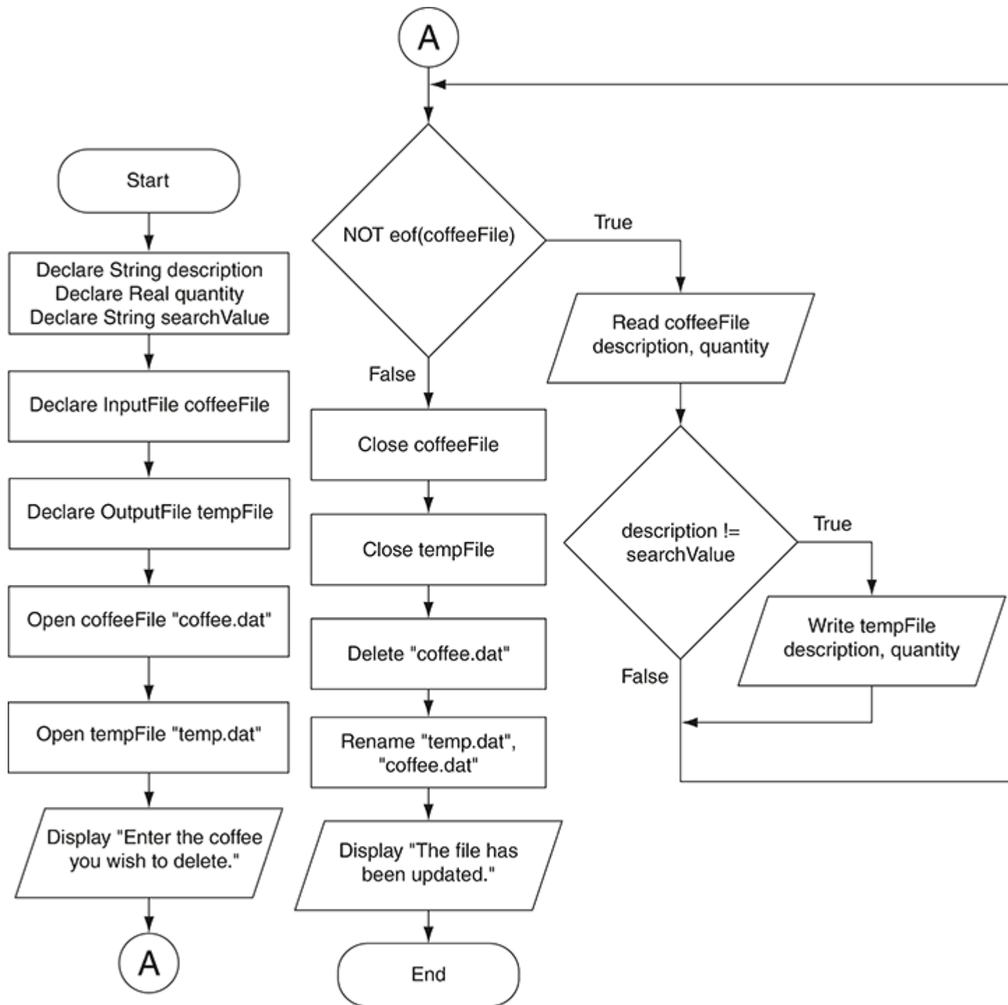
Figure 10-26 Flowchart for Program 10-13
