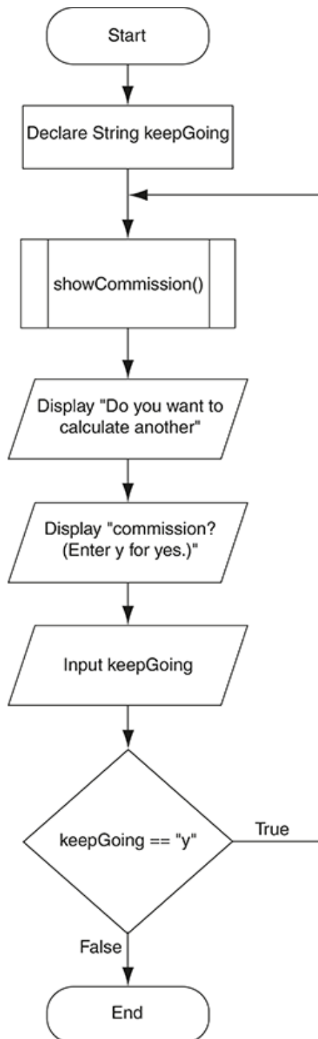
Figure 5-8 Flowchart for the main module in Program 5-5
