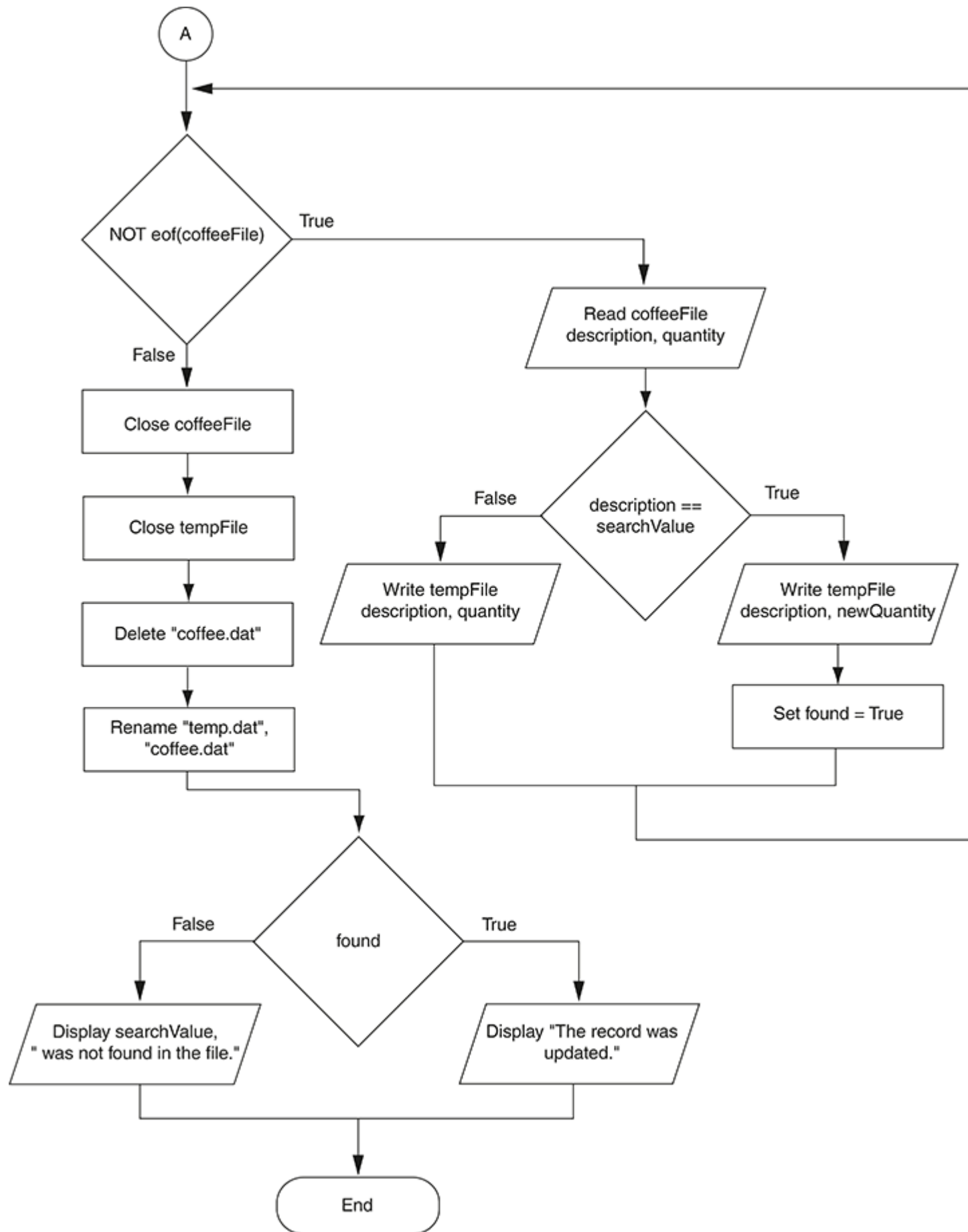
Figure 10-25 Flowchart for Program 10-12, part 2
