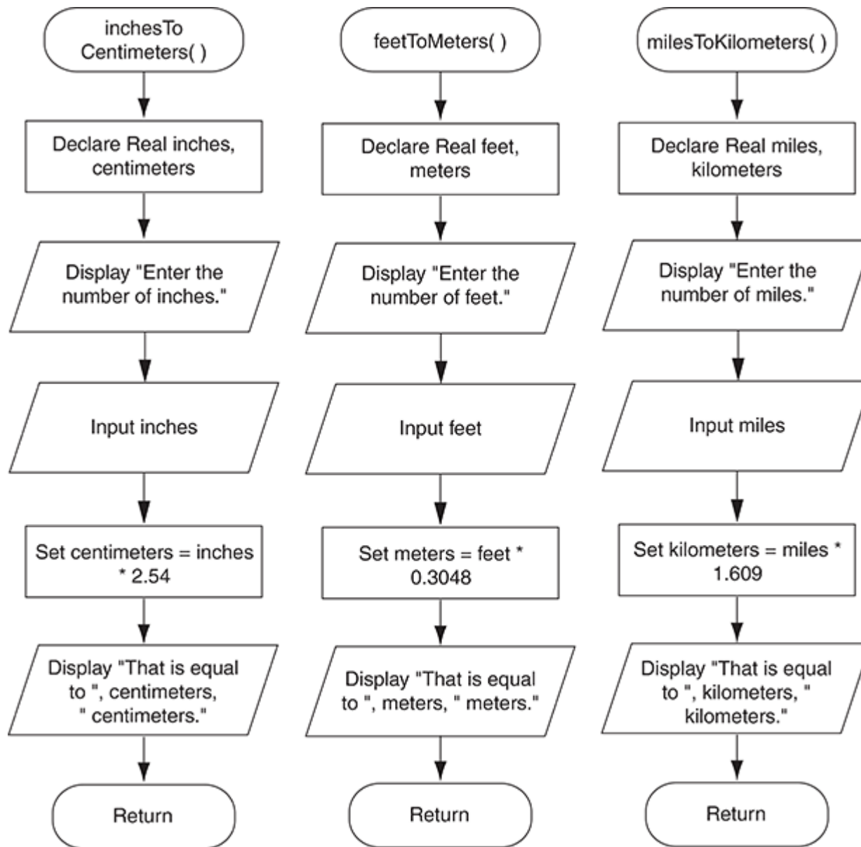
Figure 11-6 Flowcharts for the other modules in Program 11-4
