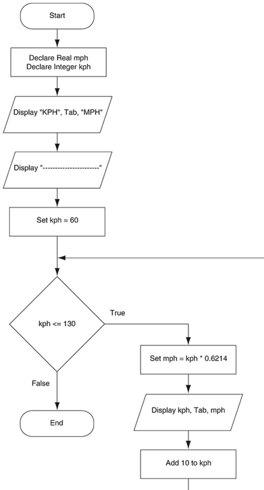
Figure 5-16 Flowchart for Program 5-11
