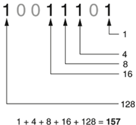
Figure 1-10 Determining the value of 10011101
