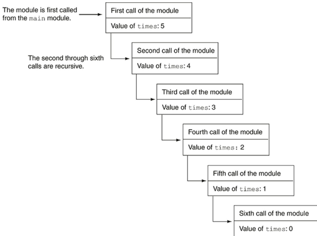
Figure 13-2 Six calls to the message module
