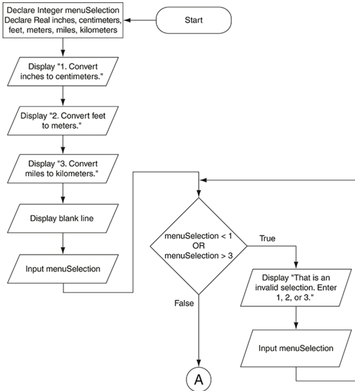
Figure 11-4 Flowchart for Program 11-3
