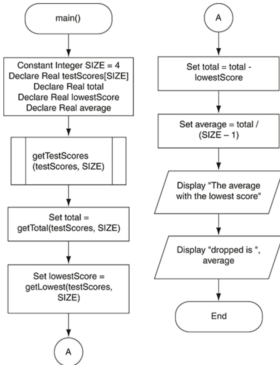
Figure 8-10 Flowchart for the main module
