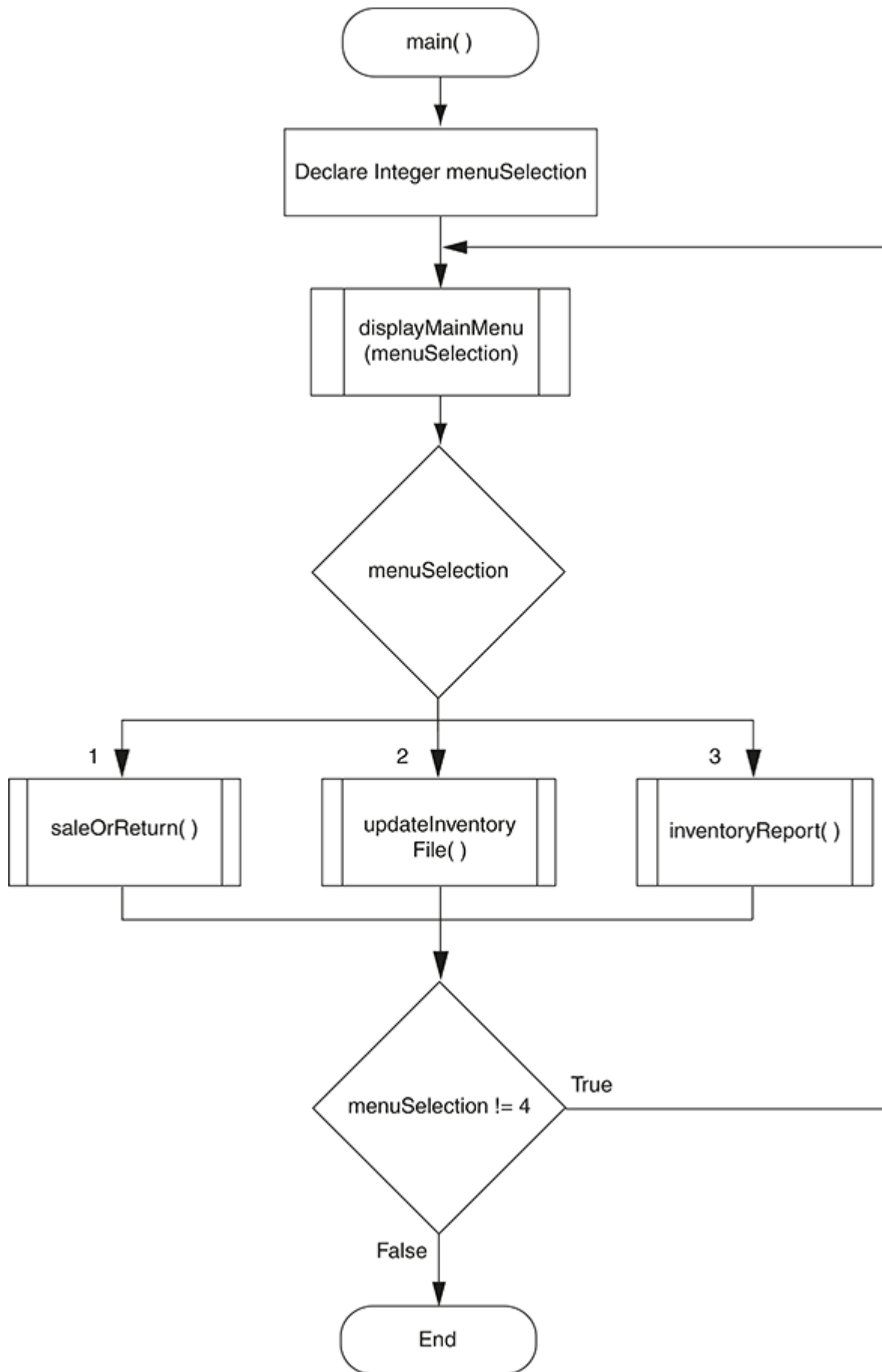
Figure 11-16 Logic for the main module
