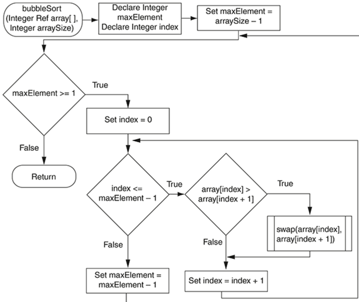
Figure 9-10 Flowchart for the bubble sort algorithm
