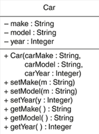
Figure 14-15 UML diagram for the Car class
