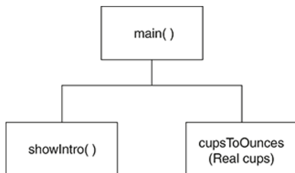
Figure 3-16 Hierarchy chart for the program
