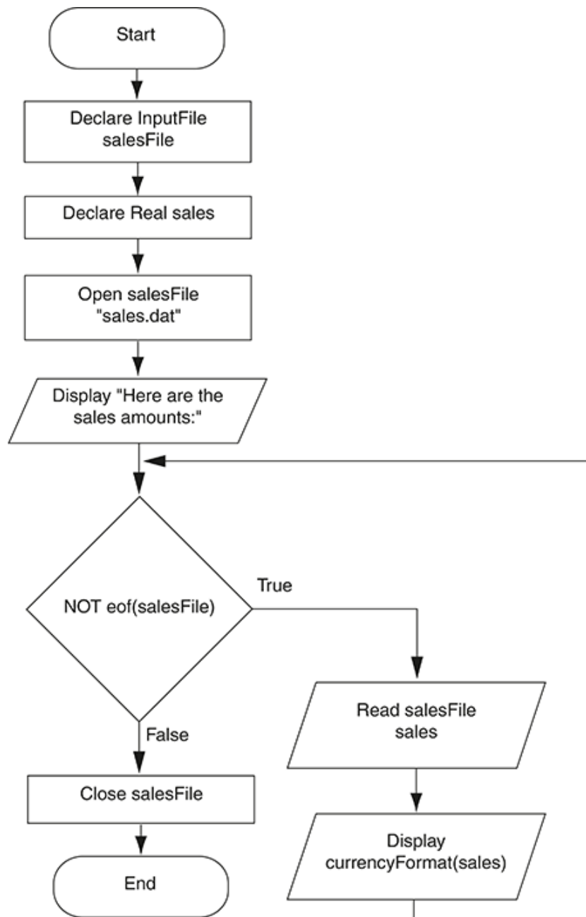
Figure 10-14 Flowchart for Program 10-4
