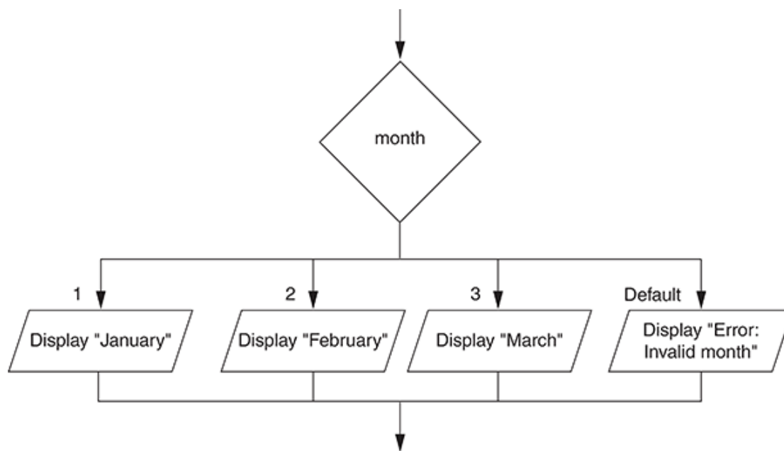
Figure 4-18 A case structure
