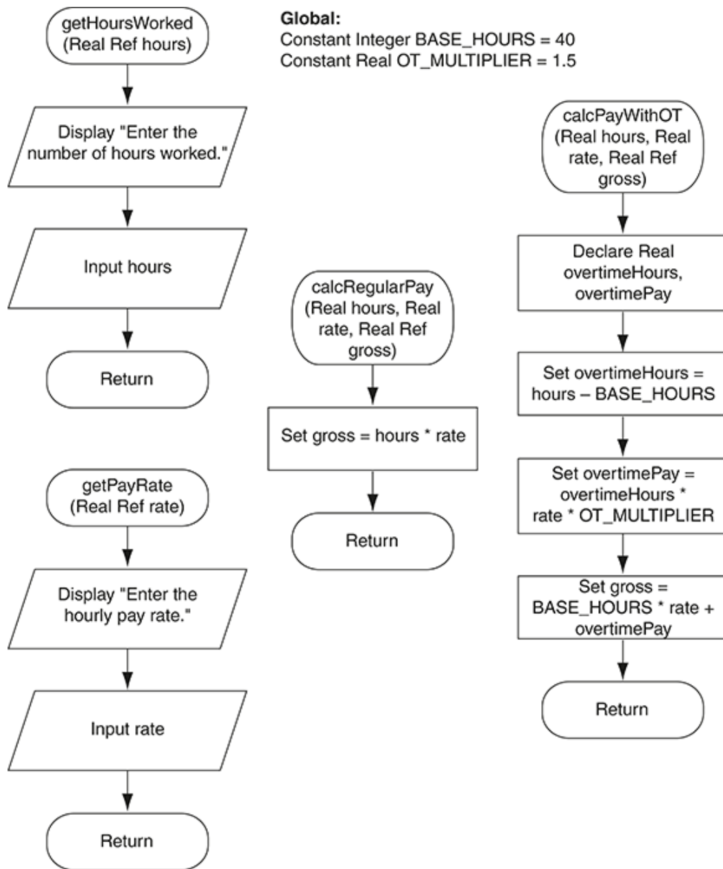
Figure 4-12 Flowcharts for the other modules
