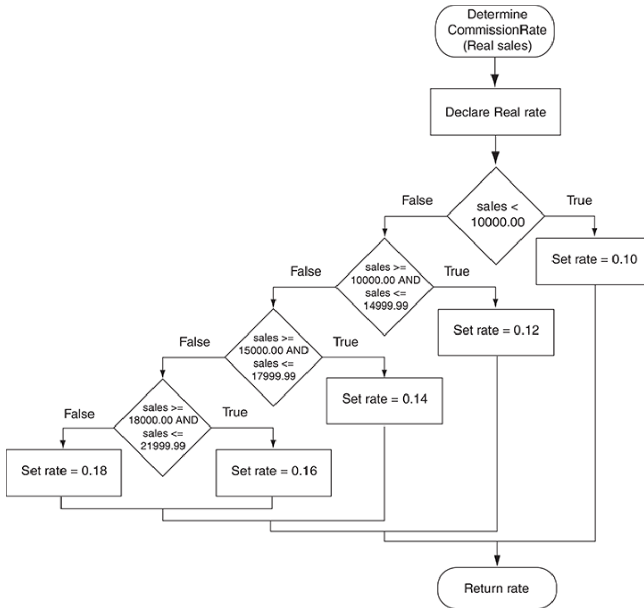
Figure 6-14 Flowchart for the determineCommissionRate function
