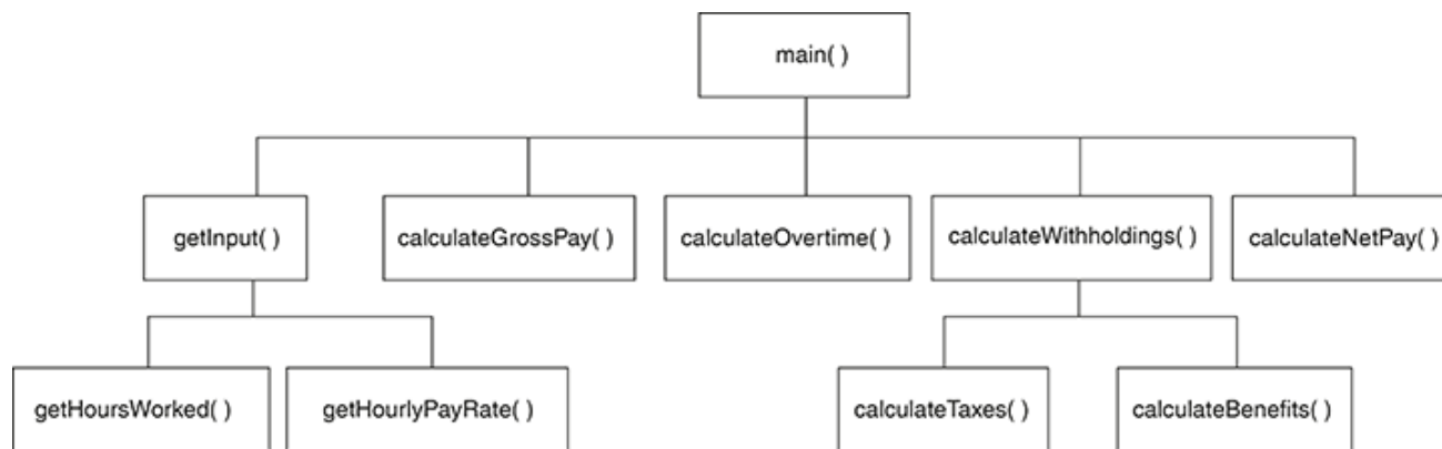
Figure 3-7 A hierarchy chart
