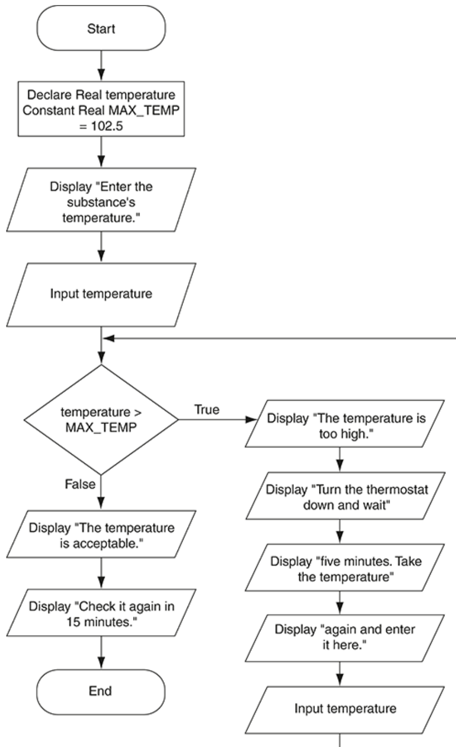
Figure 5-4 Flowchart for Program 5-2
