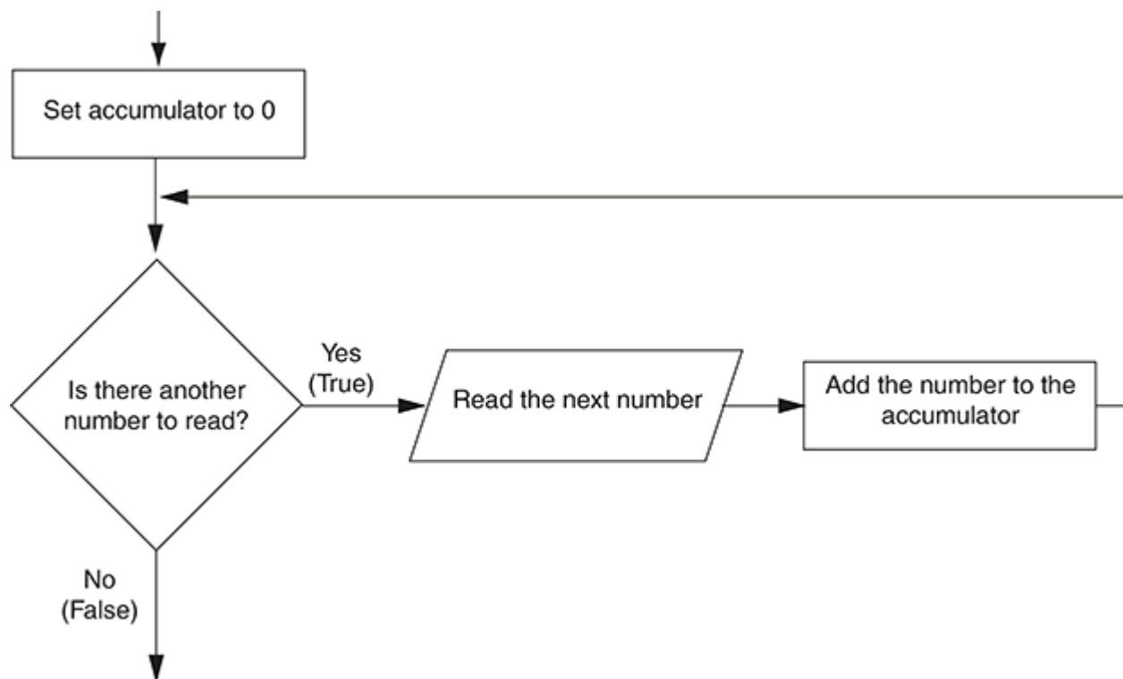
Figure 5-18 General logic for calculating a running total
