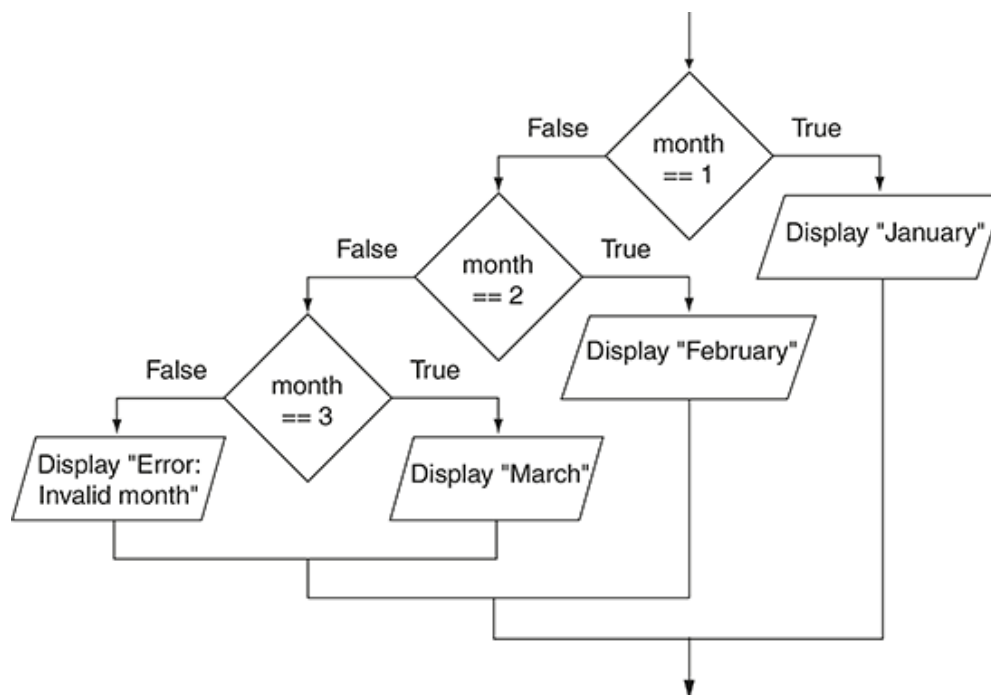
Figure 4-19 Nested decision structures
