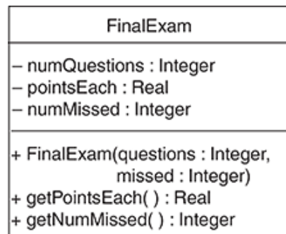
Figure 14-19 UML diagram for the FinalExam class
