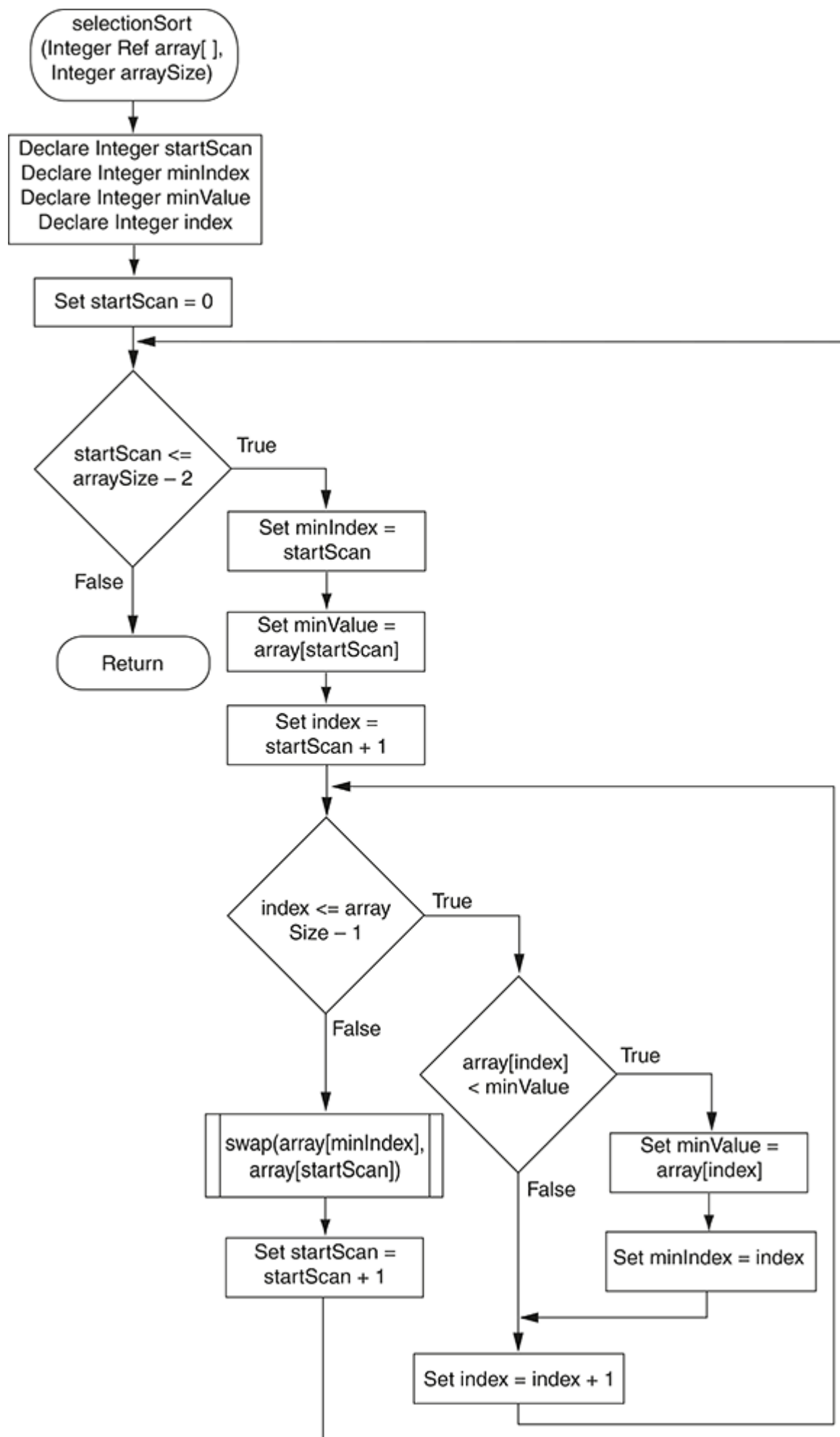
Figure 9-17 Flowchart for the selectionSort module
