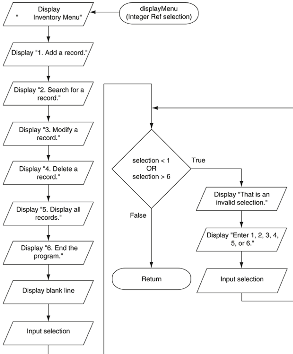
Figure 11-9 Flowchart for the displayMenu module in Program 11-6
