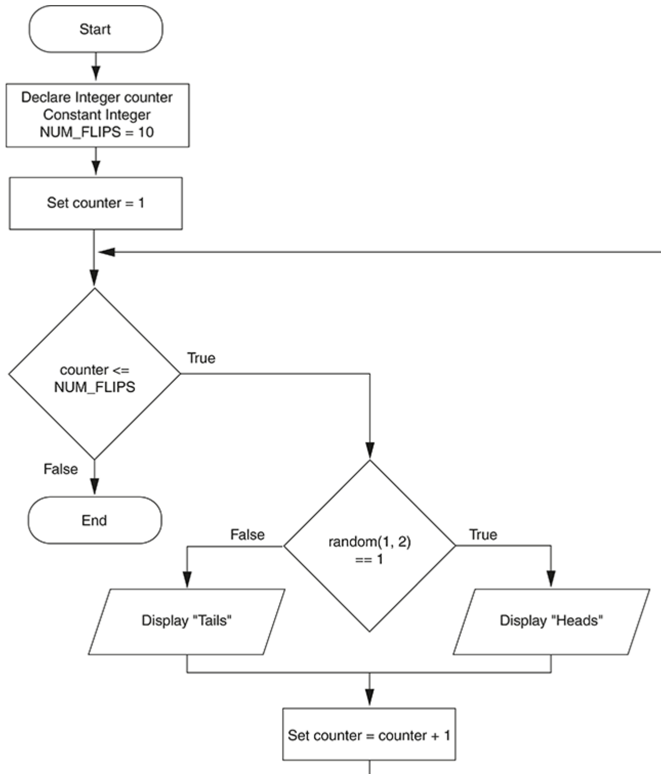
Figure 6-6 Flowchart for Program 6-5
