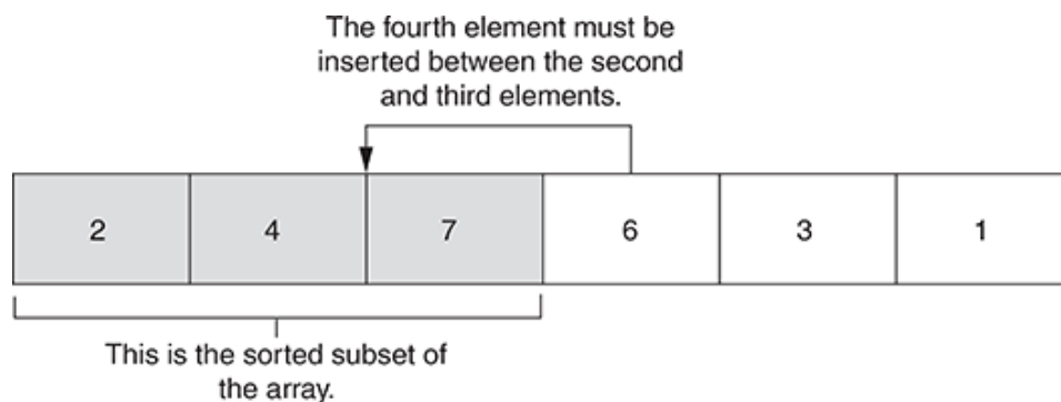
Figure 9-20 The fourth element must be moved
