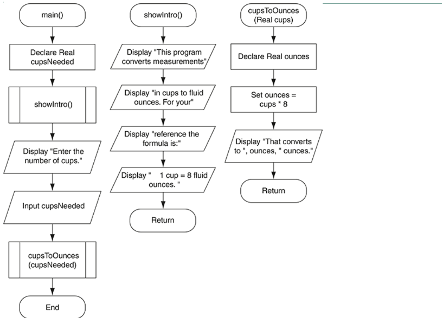
Figure 3-17 Flowchart for Program 3-8
