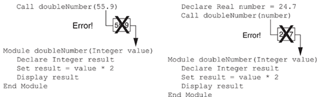
Figure 3-14 Arguments and parameter variables must be of the same type
