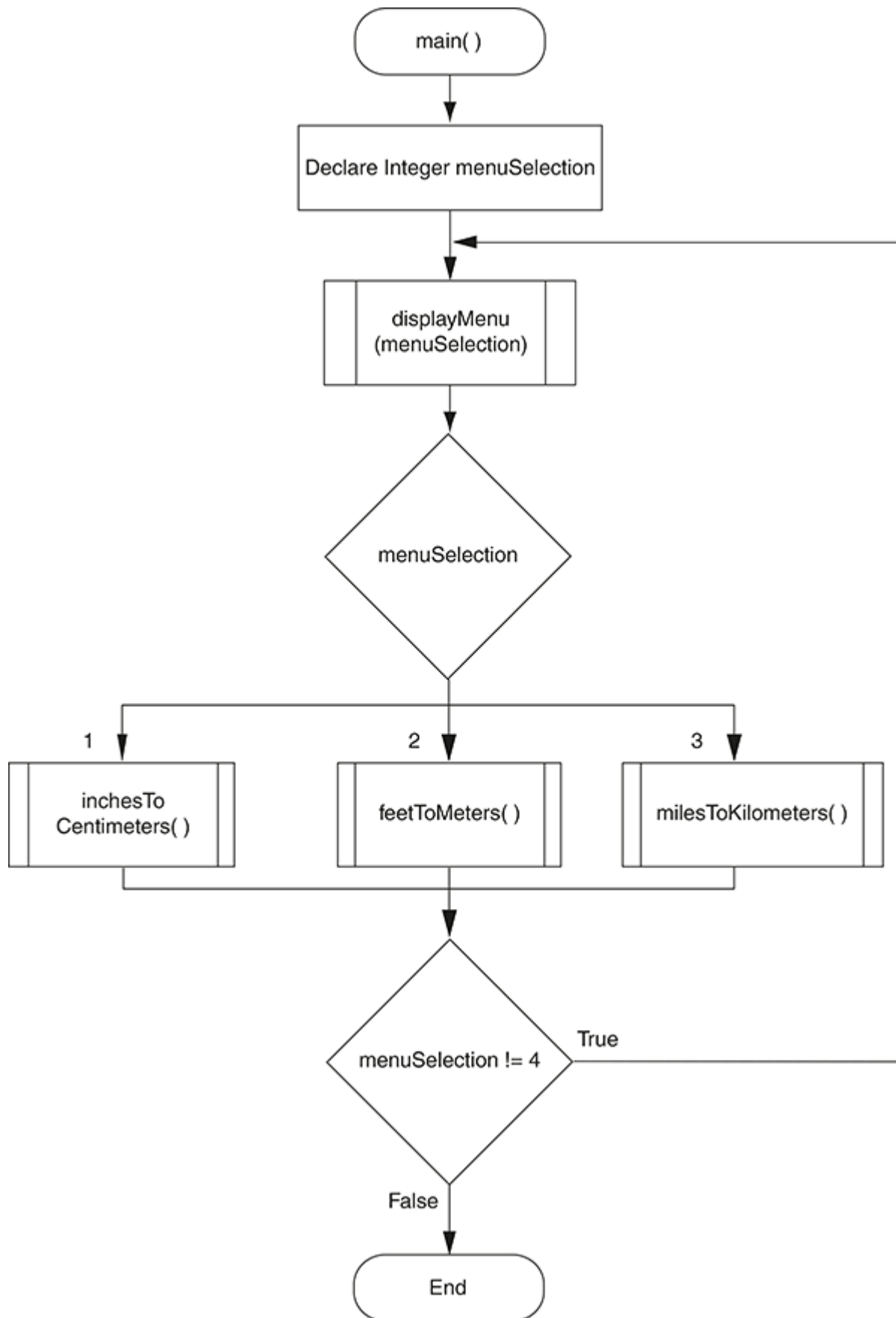
Figure 11-7 Flowchart for the main module in Program 11-5
