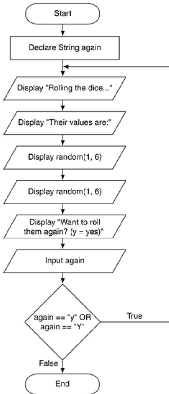
Figure 6-5 Flowchart for Program 6-4
