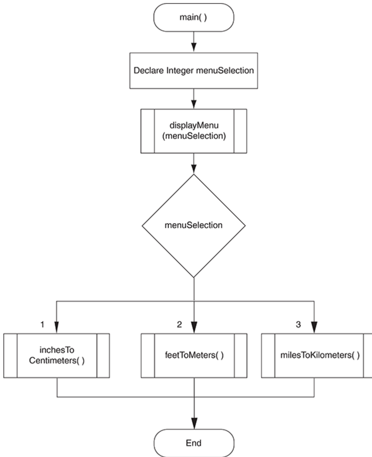
Figure 11-5 Flowchart for the main module in Program 11-4
