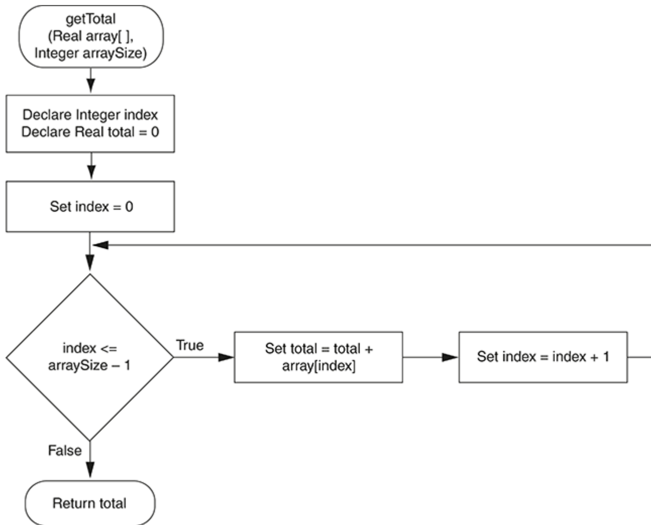
Figure 8-12 Flowchart for the getTotal function
