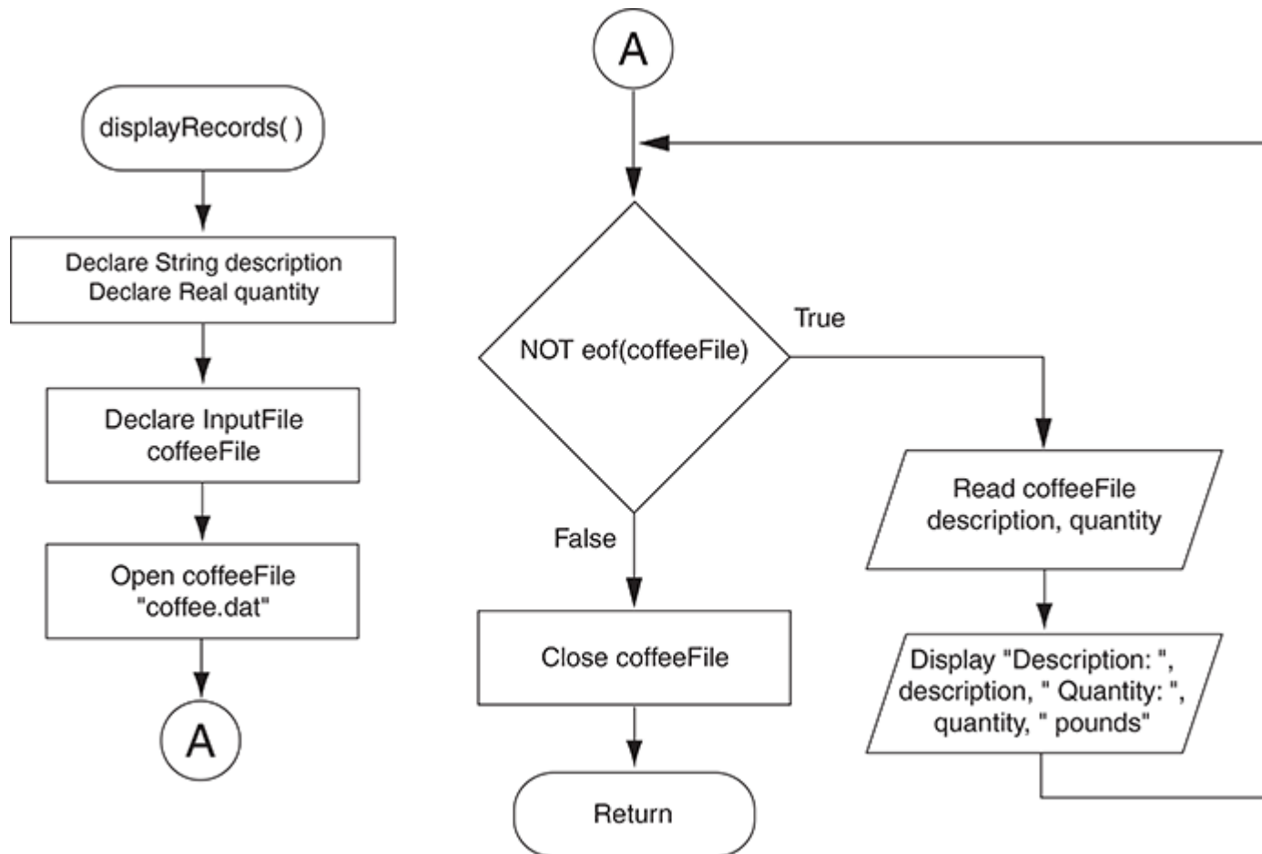
Figure 11-15 Flowchart for the displayRecords module in Program 11-6
