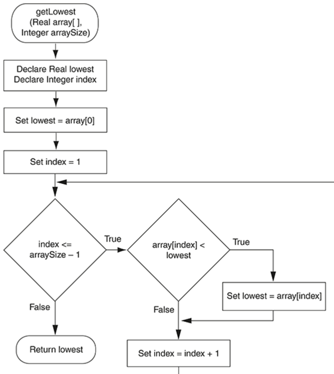
Figure 8-13 Flowchart for the getLowest function
