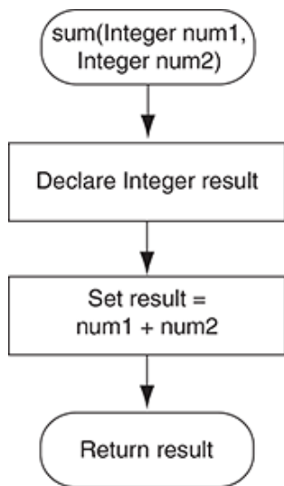
Figure 6-9 Flowchart for the sum function
