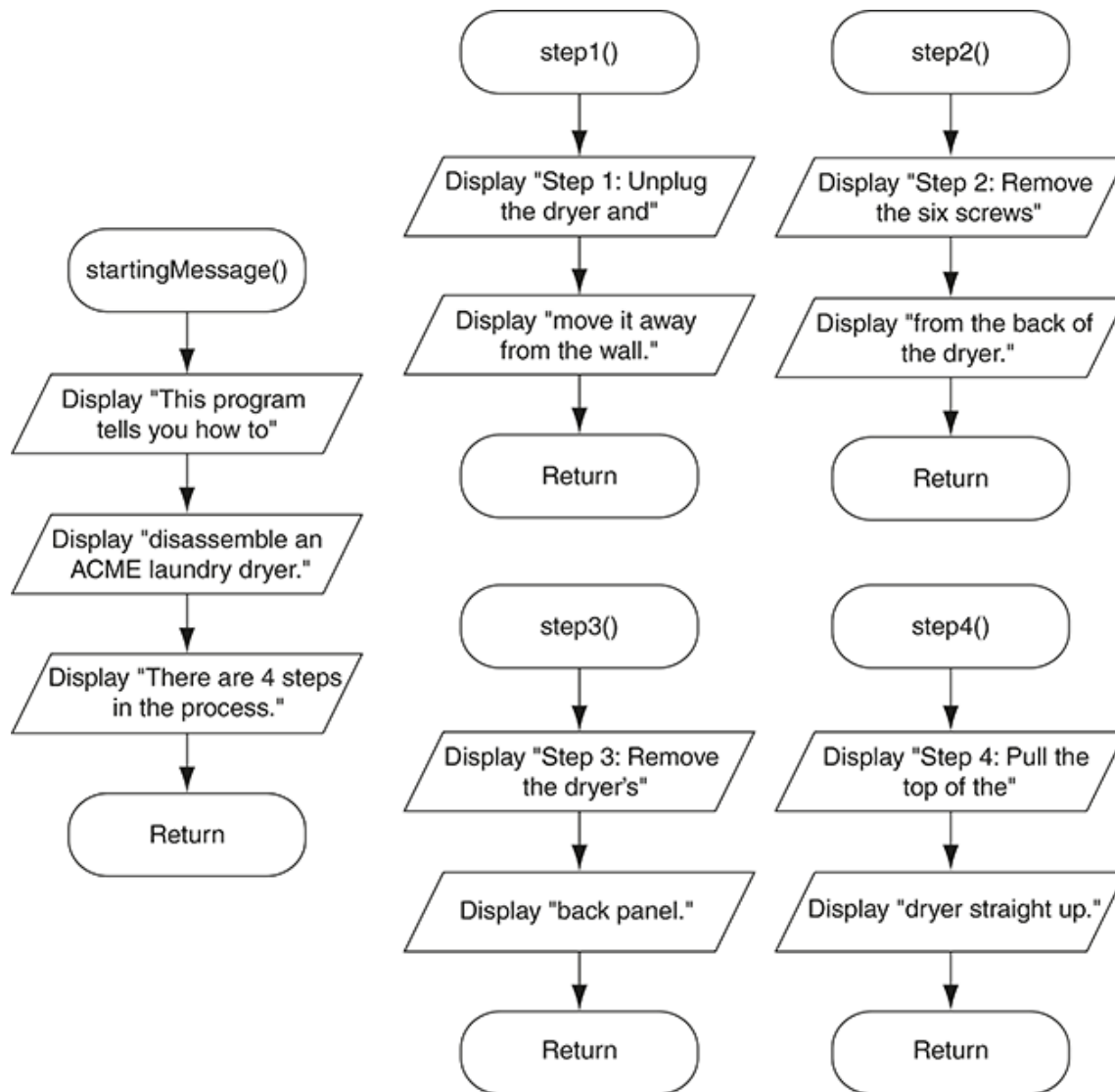
Figure 3-10 Flowcharts for the other modules in Program 3-2
