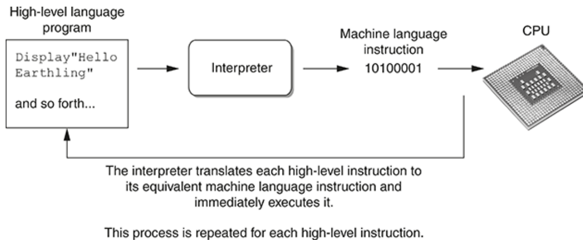
Figure 1-19 Executing a high-level program with an interpreter
