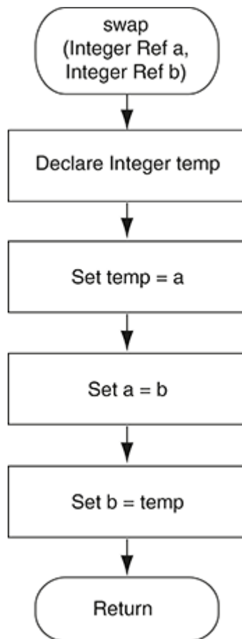
Figure 9-9 Flowchart for a swap module
