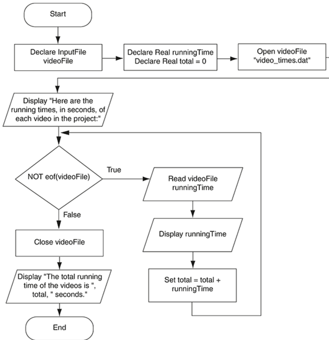
Figure 10-16 Flowchart for Program 10-6
