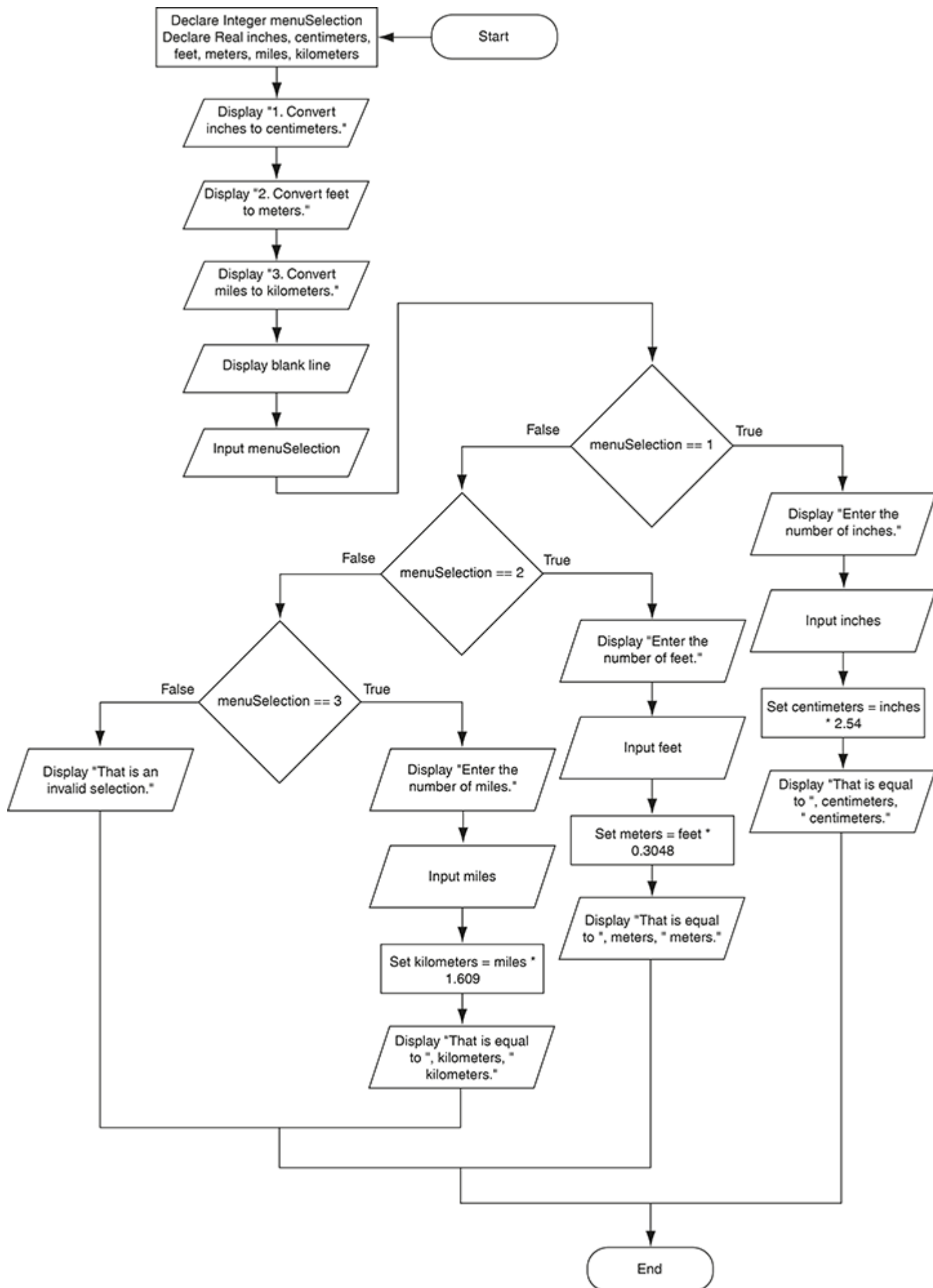
Figure 11-3 Flowchart for Program 11-2
