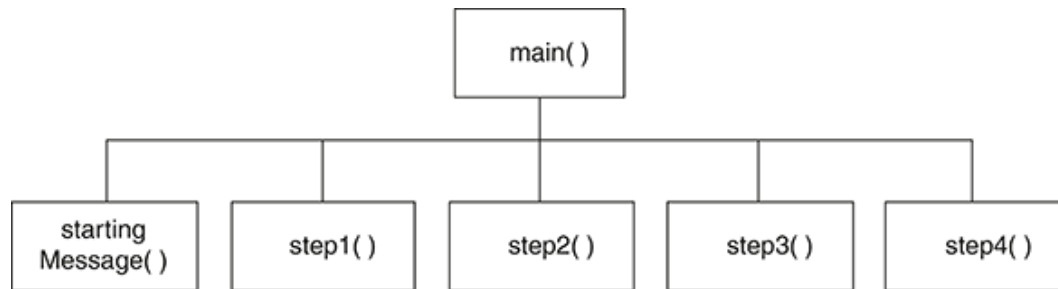
Figure 3-8 Hierarchy chart for the program
