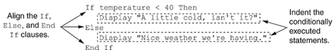
Figure 4-9 Programming style with an If-Then-Else statement
