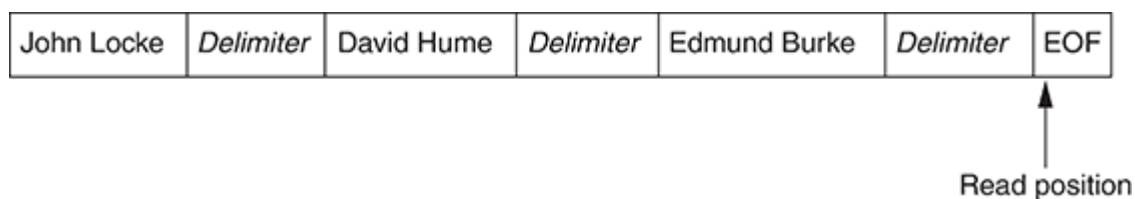
Figure 10-11 Read position after the third Read statement
