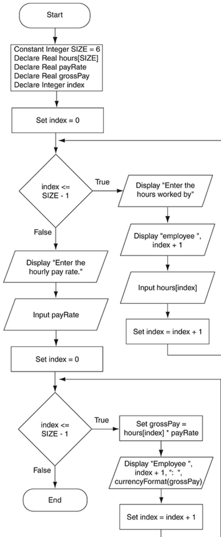
Figure 8-4 Flowchart for Program 8-4
