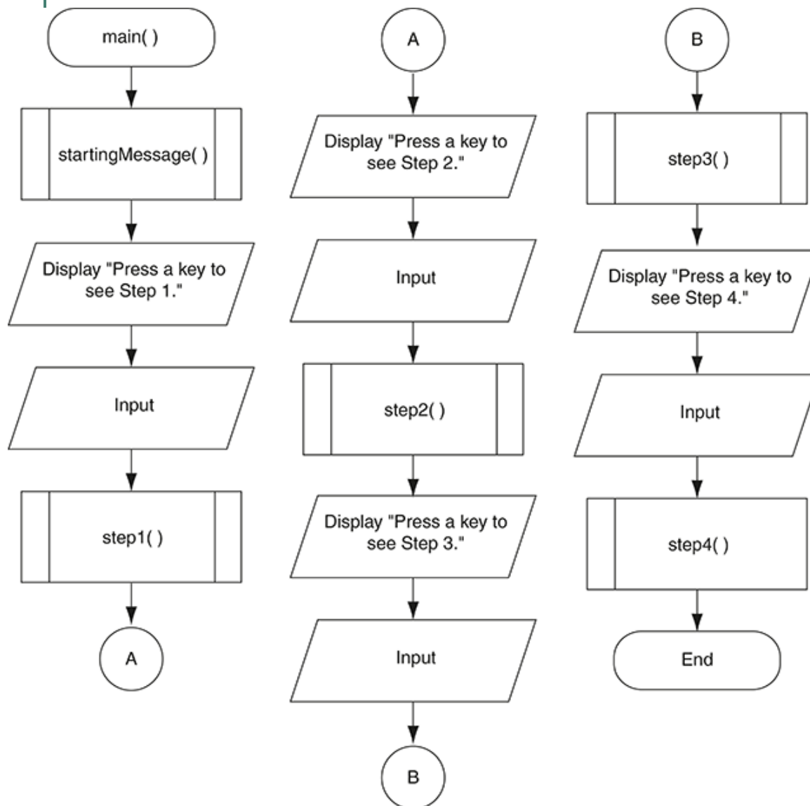
Figure 3-9 Flowchart for the main module in Program 3-2
