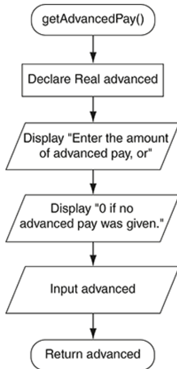
Figure 6-13 Flowchart for the getAdvancedPay function
