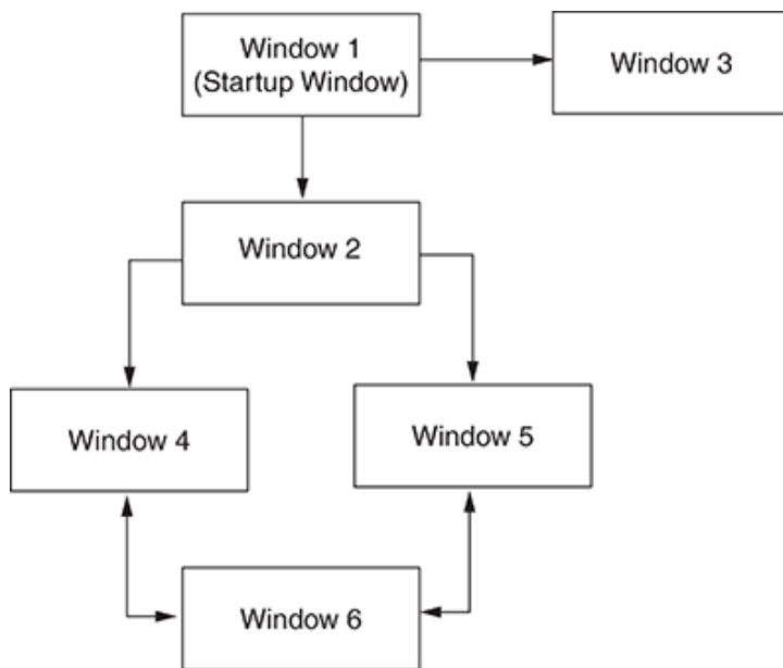
Figure 15-4 A user interface flow diagram
