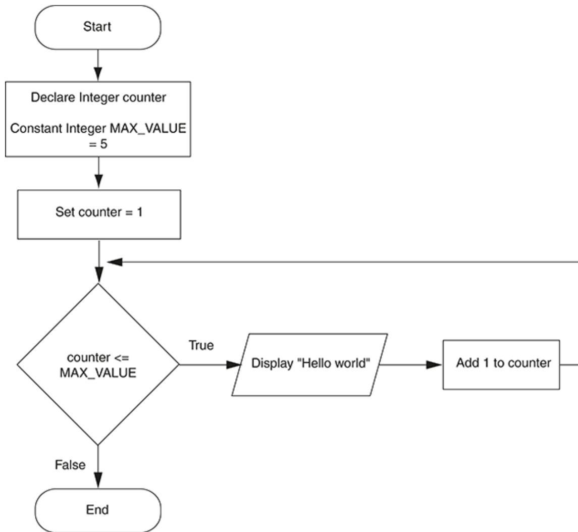
Figure 5-14 Flowchart for Program 5-8
