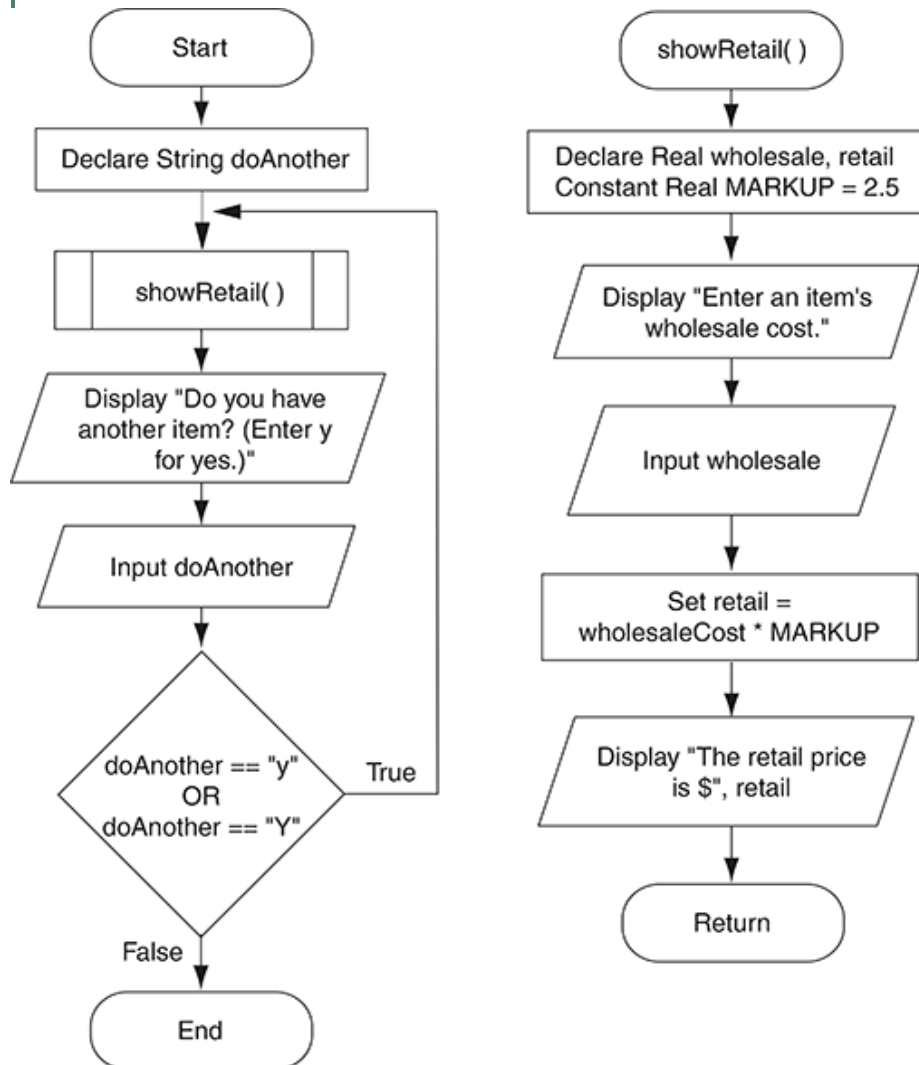
Figure 5-9 Flowchart for Program 5-6
