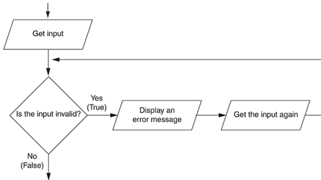
Figure 7-1 Logic containing an input validation loop
