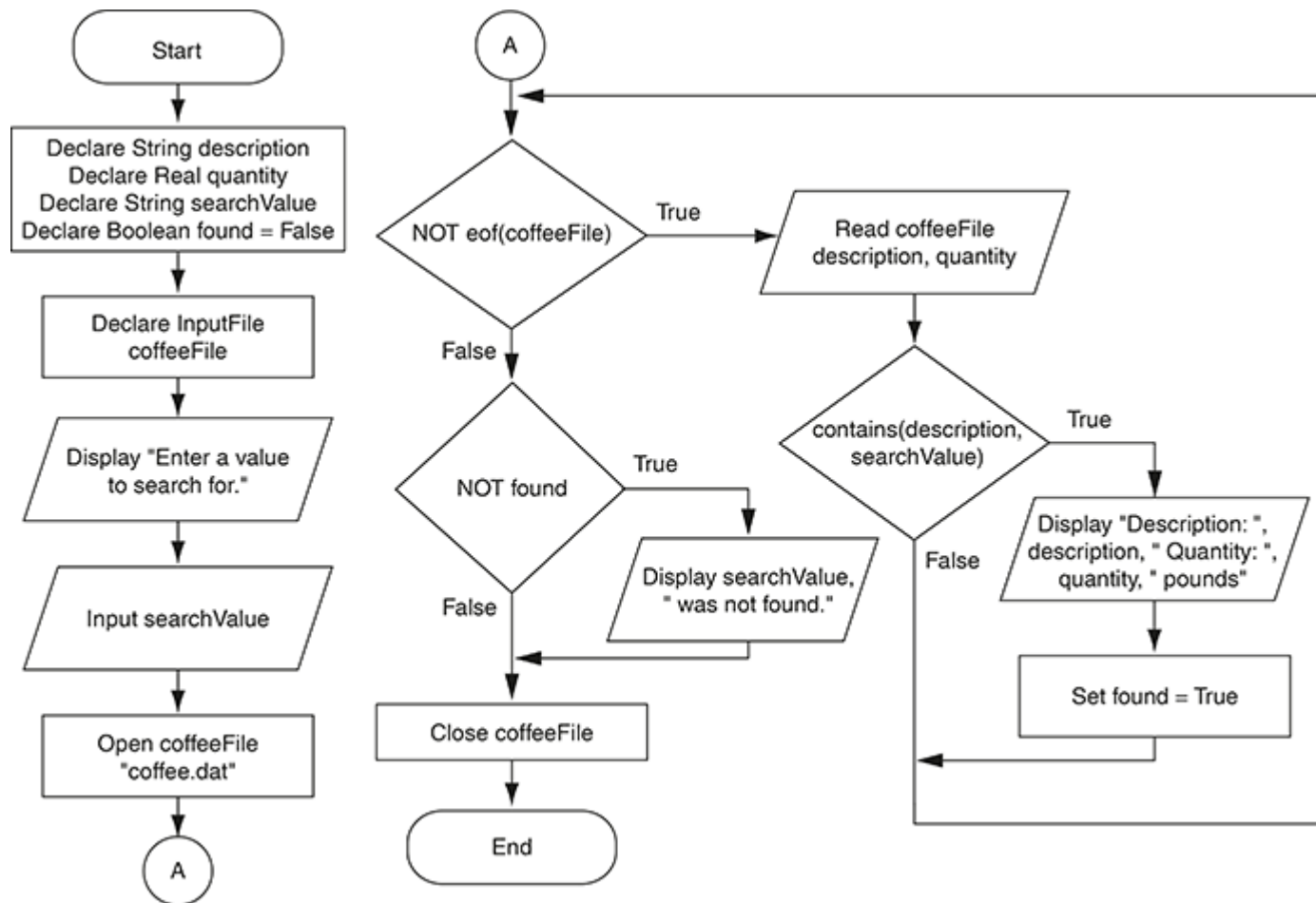
Figure 10-23 Flowchart for Program 10-11
