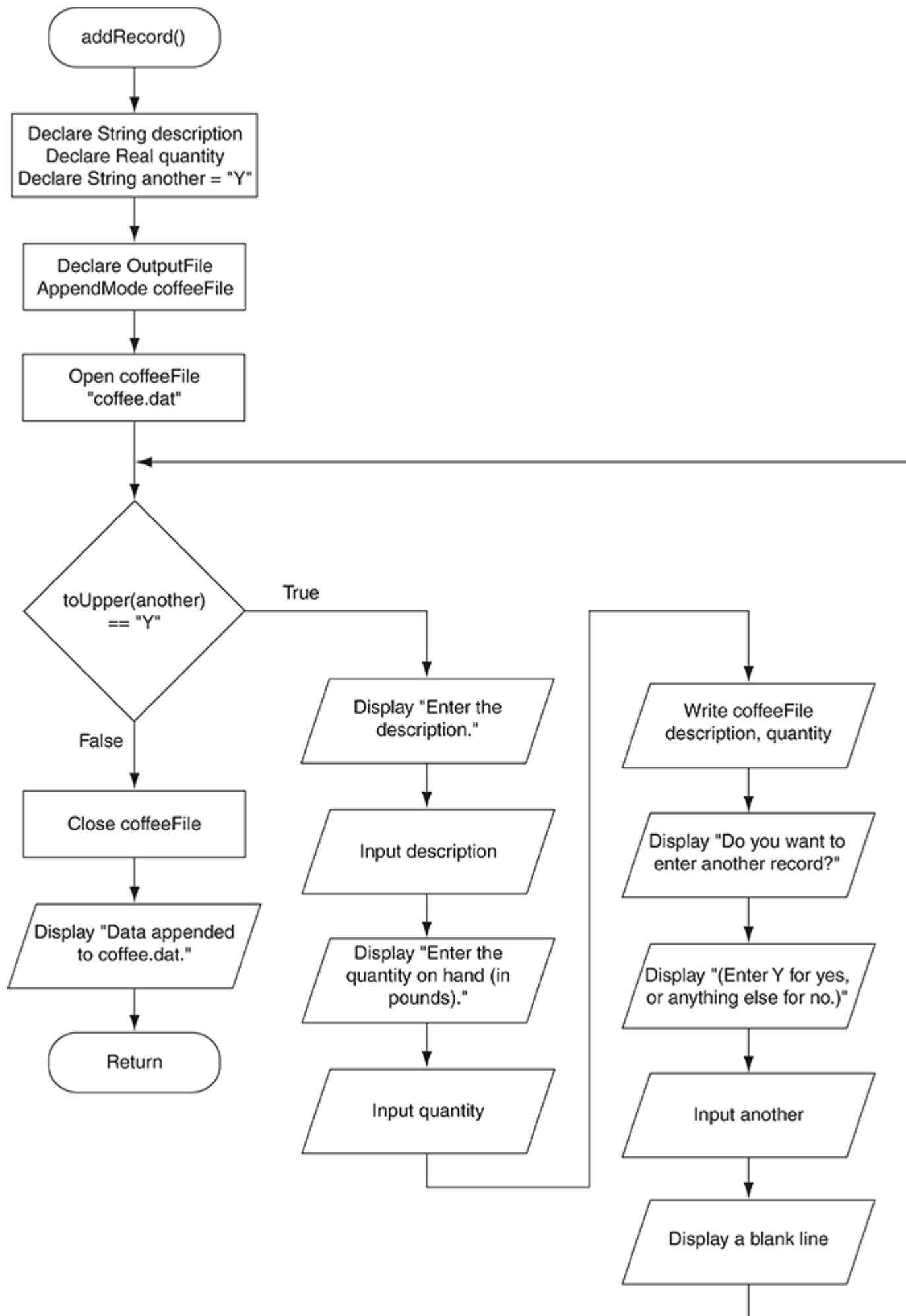
Figure 11-10 Flowchart for the addRecord module in Program 11-6
