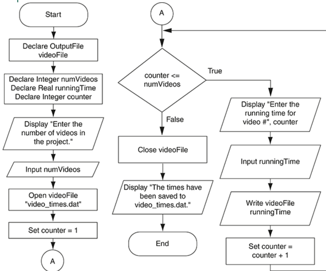
Figure 10-15 Flowchart for Program 10-5
