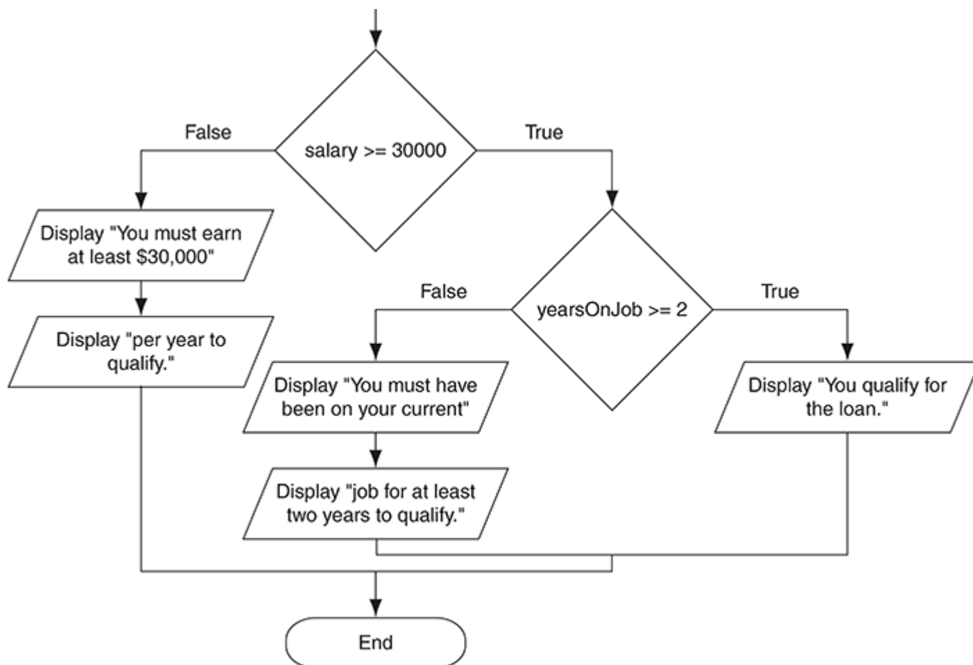
Figure 4-15 A nested decision structure
