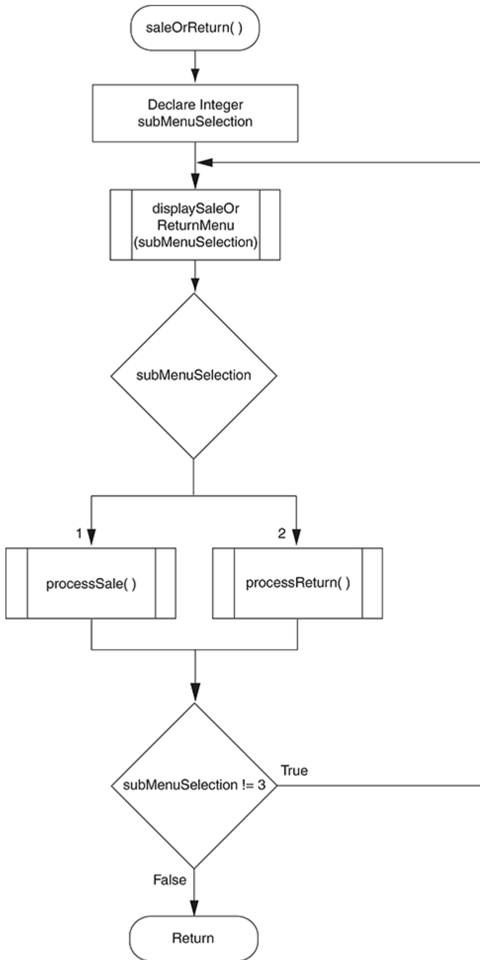
Figure 11-17 Logic for the saleOrReturn module
