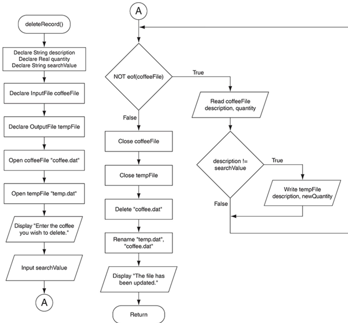
Figure 11-14 Flowchart for the deleteRecord module in Program 11-6
