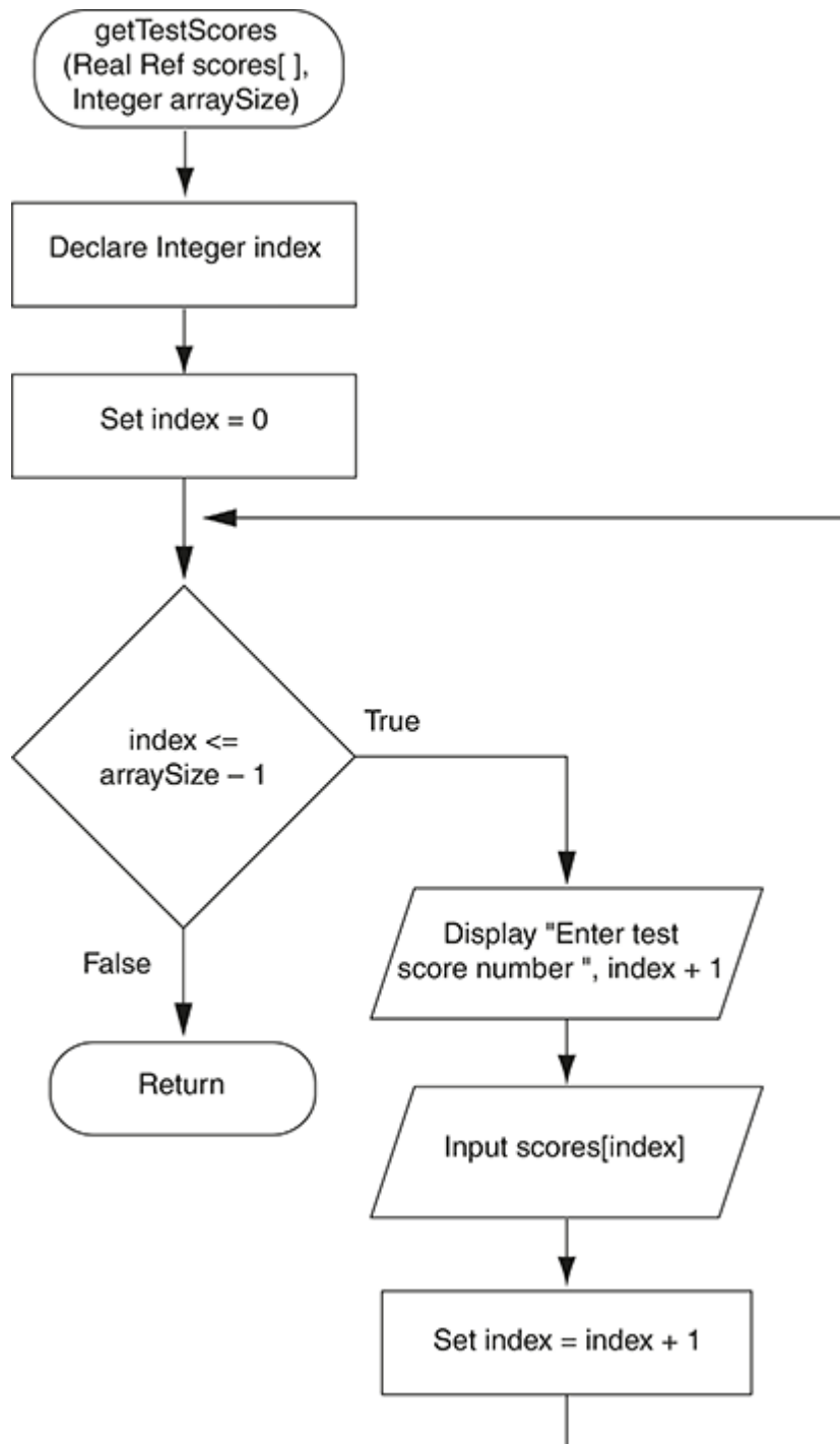
Figure 8-11 Flowchart for the getTestScores module
