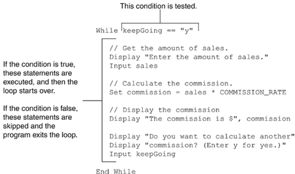
Figure 5-2 The While loop
