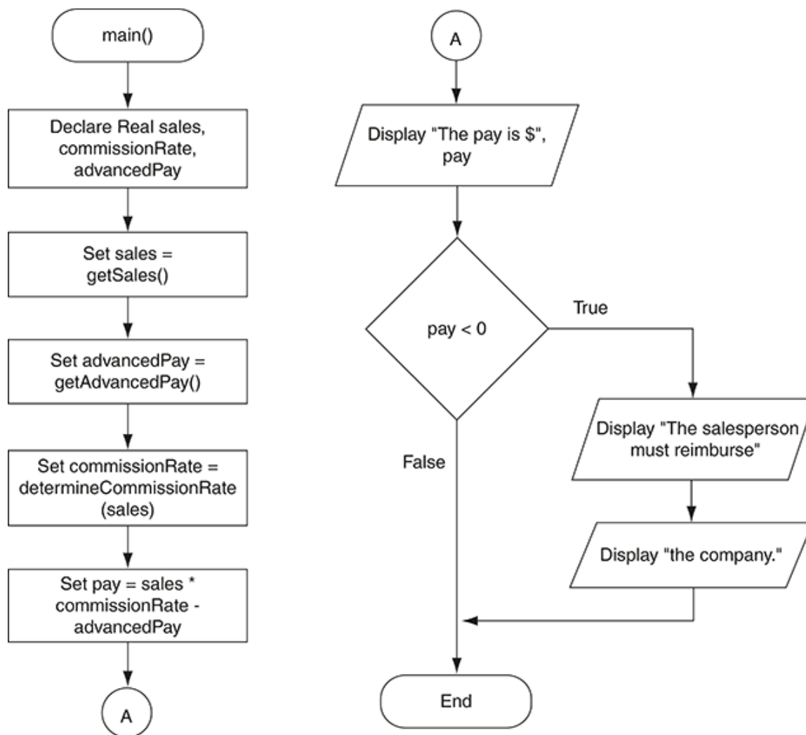
Figure 6-11 Flowchart for the main module
