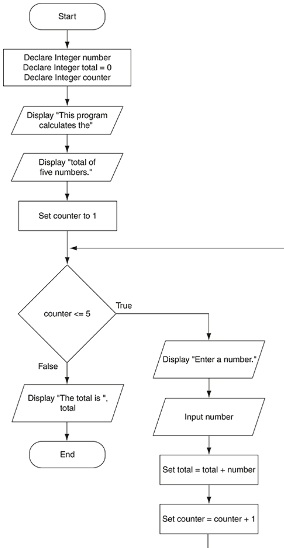
Figure 5-19 Flowchart for Program 5-18
