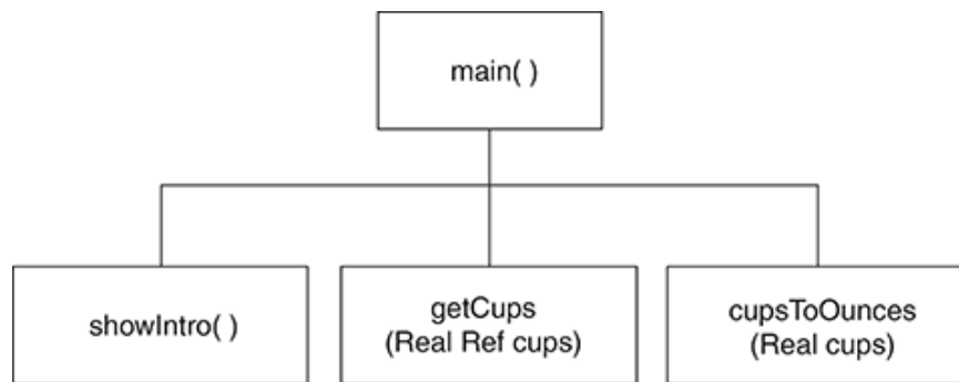
Figure 3-18 Revised hierarchy chart
