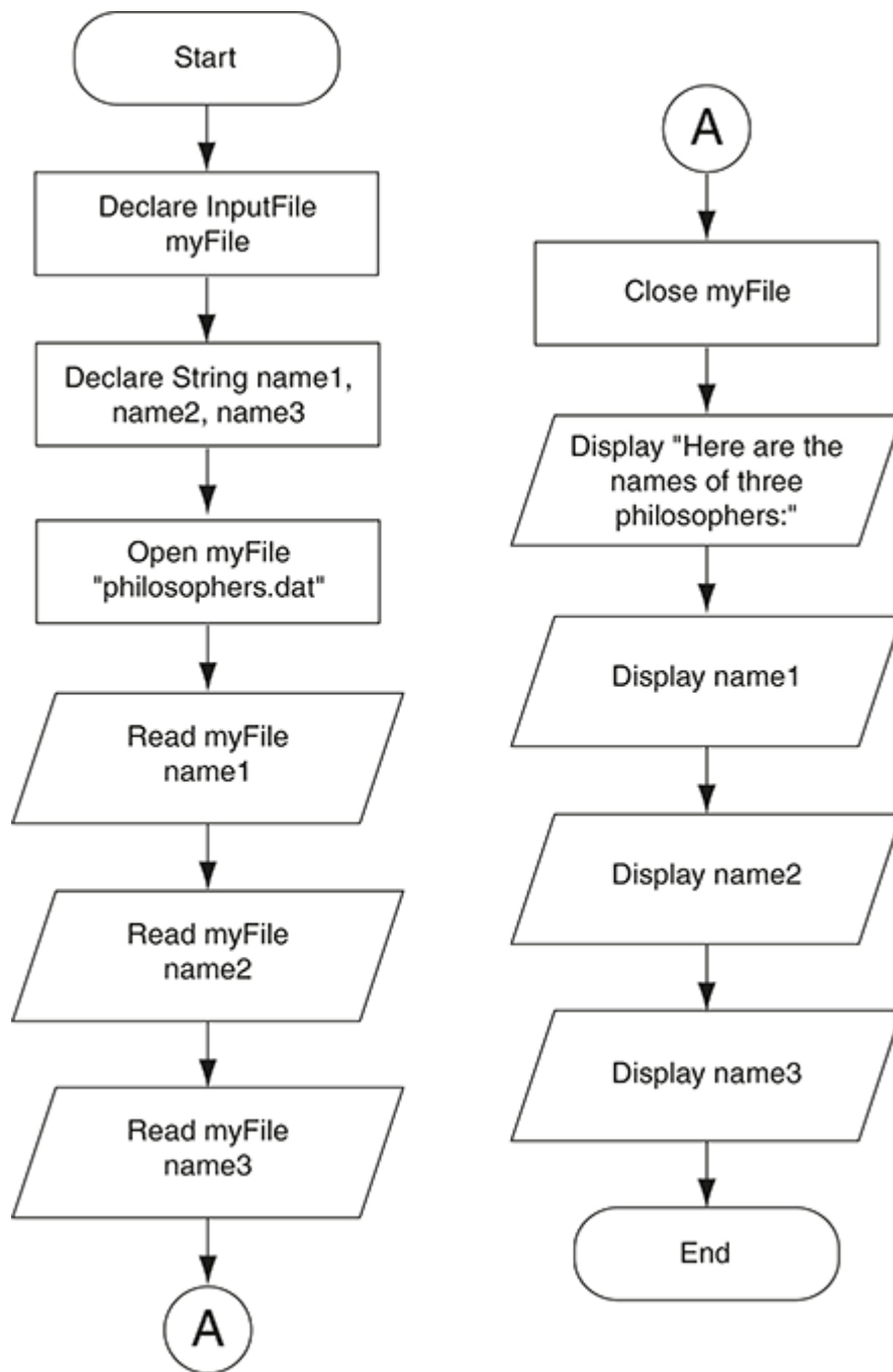
Figure 10-7 Flowchart for Program 10-2
