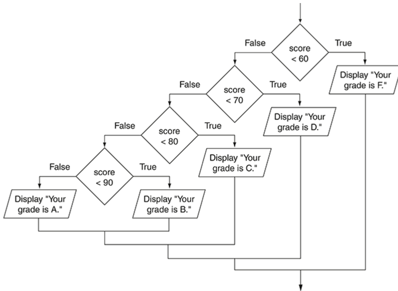
Figure 4-17 Nested decision structure to determine a grade
