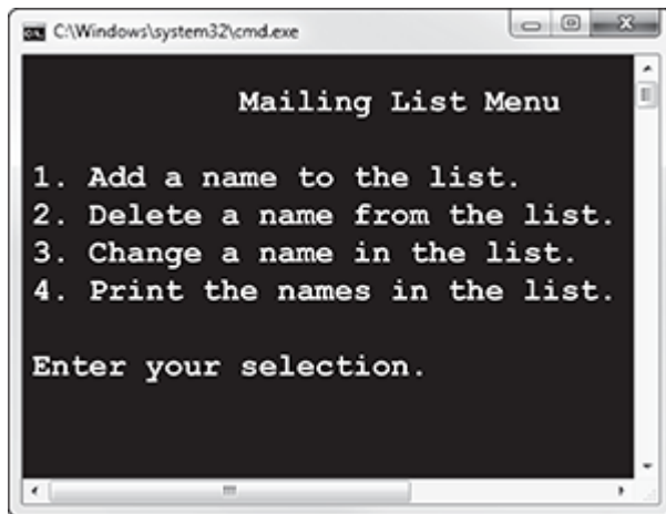
Figure 11-1 A menu
