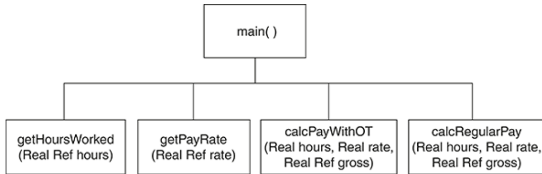
Figure 4-10 Hierarchy chart
