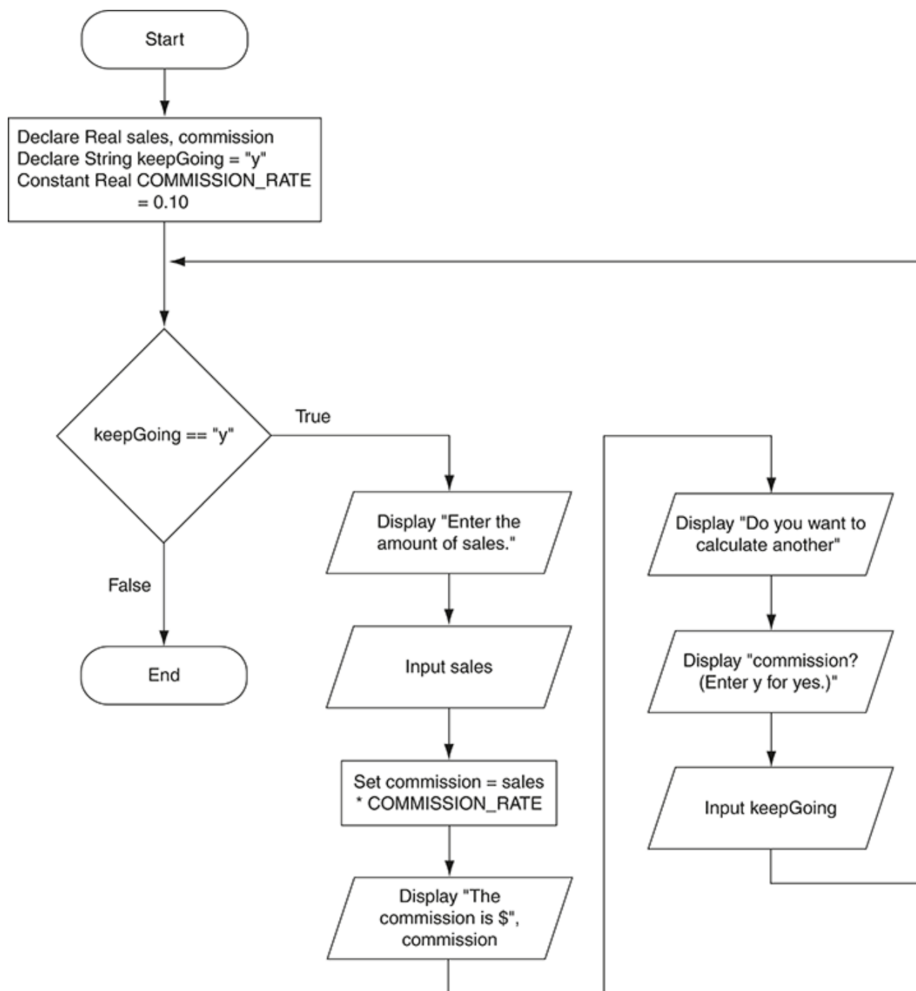
Figure 5-3 Flowchart for Program 5-1
