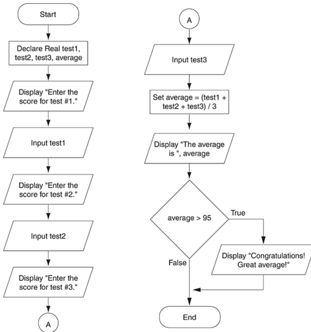
Figure 4-7 Flowchart for Program 4-1
