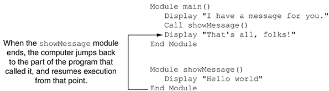
Figure 3-4 The showMessage module returns
