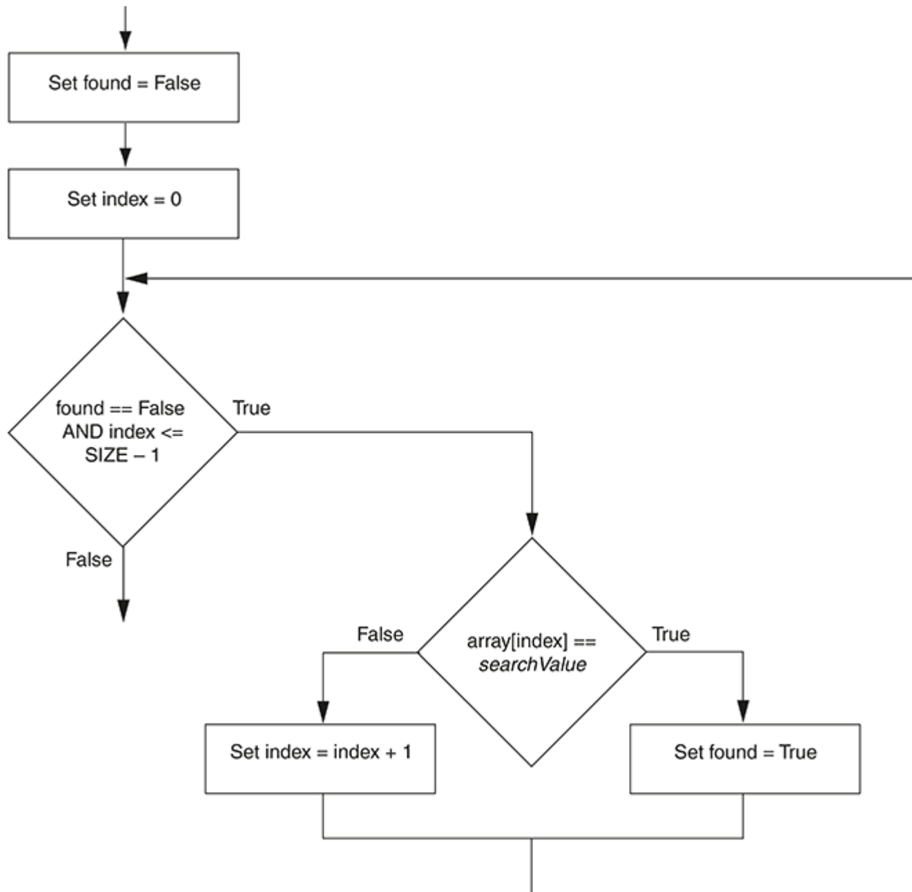
Figure 8-5 Sequential search logic
