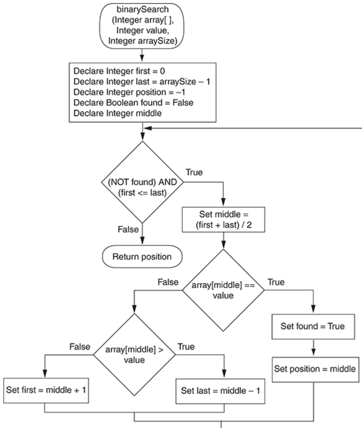
Figure 9-25 Flowchart for the binarysearch function
