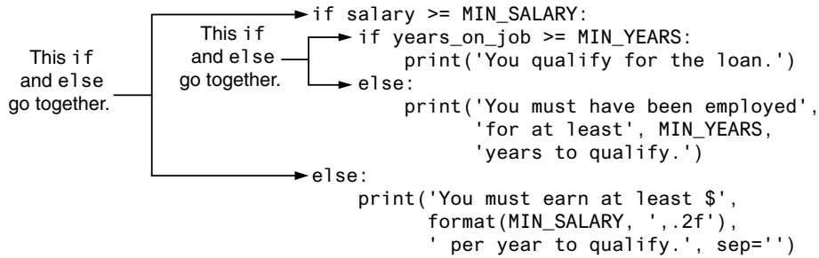
Figure 3-14 Nested blocks
